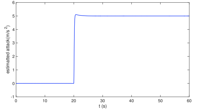
Fig. 4. The estimated attack by use of the adaptive sliding mode observer. As the threshold is equal to 0.24, we can see that detection is almost instantaneous.
