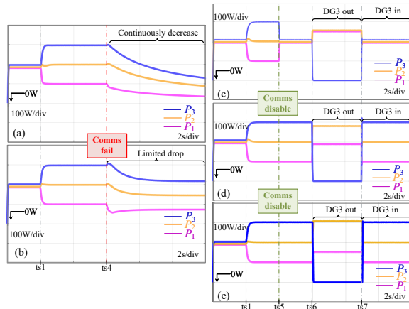
Fig. 4: Active power performance comparison: (a) DAPI in [19] without constraints. (b) the proposed DMPC. (c) plug-and-Play test of DMPC in [10]. (d) plug-and-Play test of DMPC in [24]. (e) plug-and-play test of the proposed DMPC.
