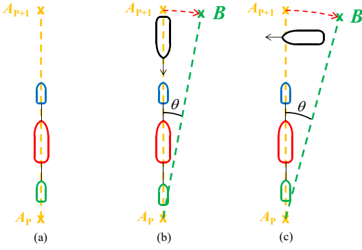
Fig. 3. Ship reference scheme: (a) under normal condition; (b) under the head-on situation; (c) under the crossing situation.
