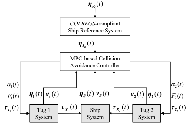
Fig. 1. System control diagram.
