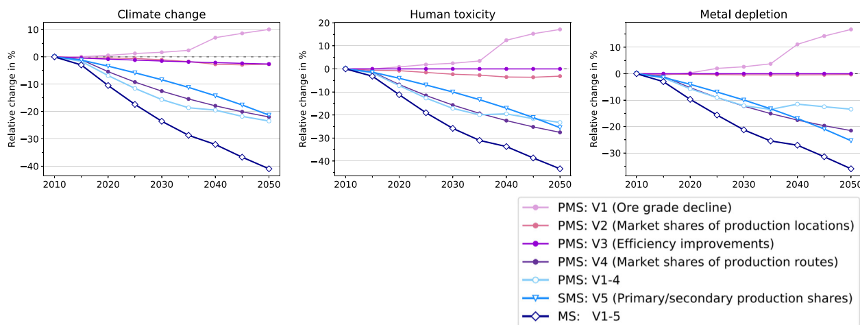
FIGURE 5 Prospective LCA results for the global market of copper: effect of variables 1 to 5
