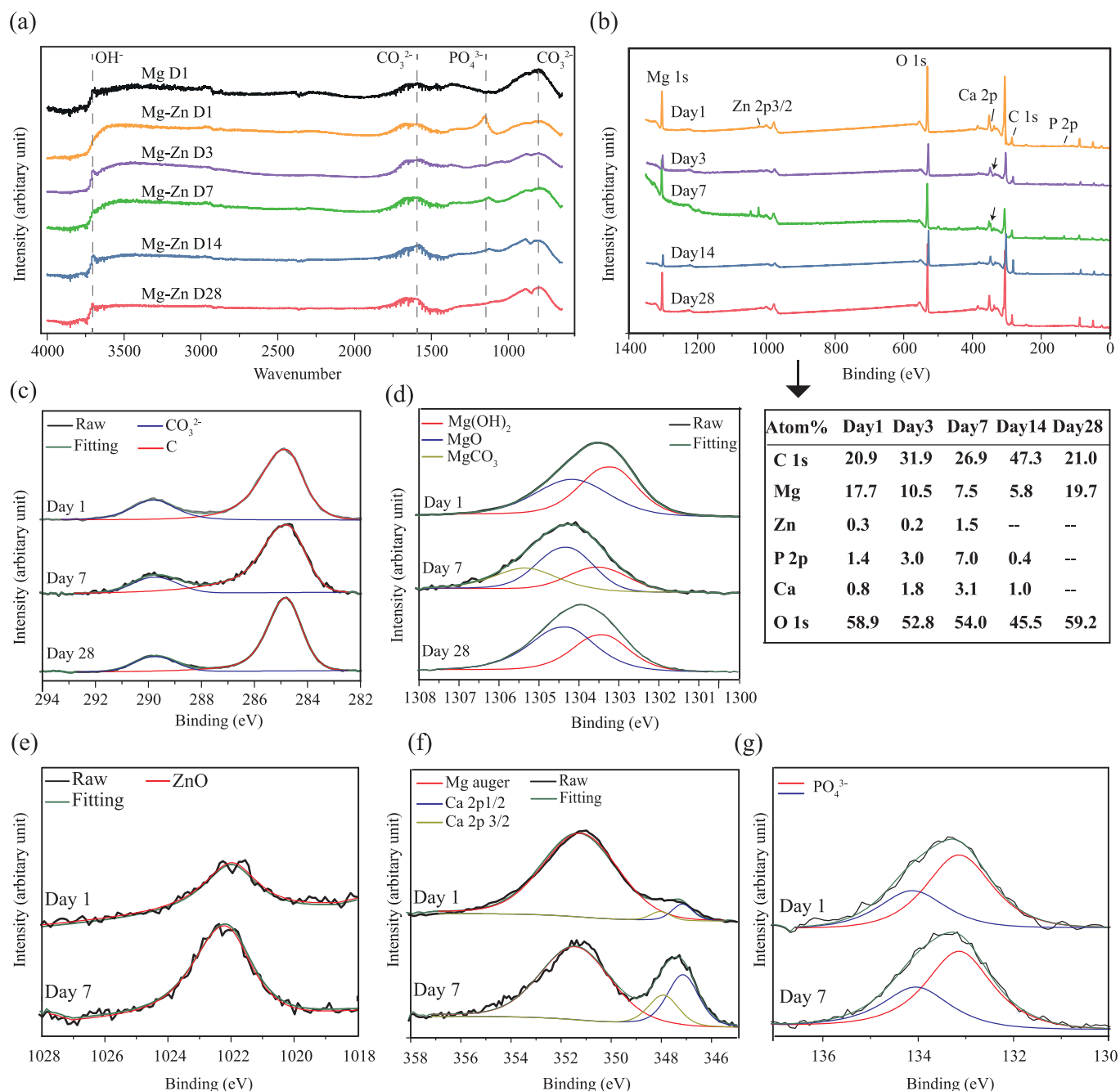
Fig. 4. Characteristics of the biodegradation products on the surface of Mg-Zn scaffold struts: (a) FTIR spectra (the spectrum of pure Mg after the first day of immersion cited from [18]), and (b-g) XPS spectra.
