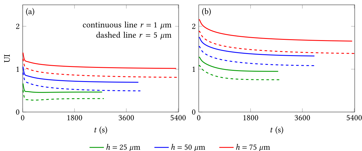
Fig. 4. Time evolution of the uniformity index (25). The performance indicator is evaluated for (a) positive and (b) negative electrode-SPE interfaces. Simulations performed with the purely electrochemical model. A uniform electric current density distribution, corresponding to \text{UI} = 0 according to (24) and (25), is approached in batteries with smaller h and larger r . The uniform current distribution is better approached along the \text{LiCoO}_2/\text{SPE} interface (a) than along the \text{C}_6/\text{SPE} interface (b), irrespective of the cell geometry.
