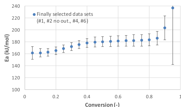
Fig. 12. Activation energies and standard deviations along conversion (KAS method) for selected cases #1, #2 (without outlier at 1 K/min), #4 and #6 for beech wood pyrolysis.
