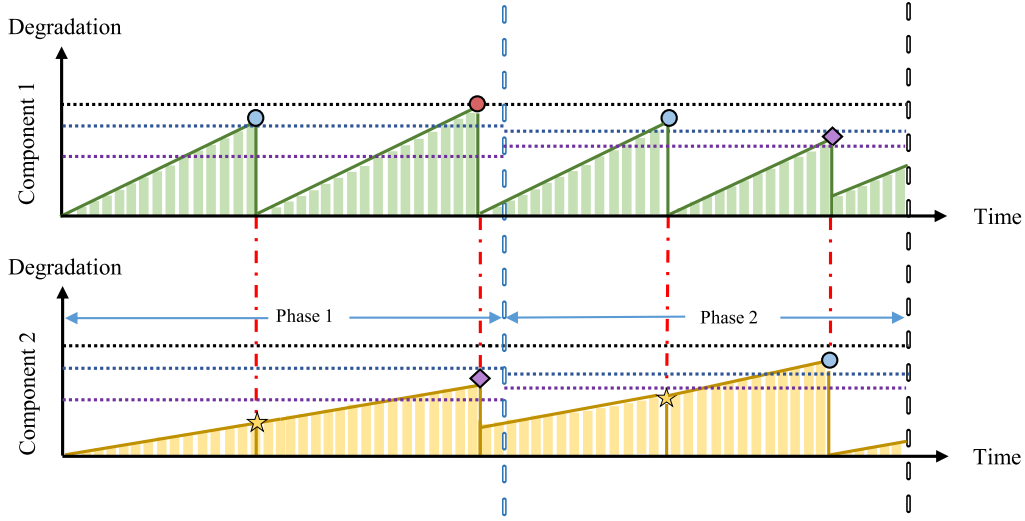
(b) Adjusting the maintenance strategy between phase 1 and 2
