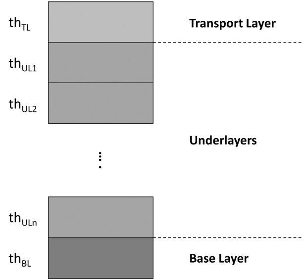
FIGURE 1 Multi-layer administration in Delft3D, consisting of a transport layer, n numbers of underlayers, and a base layer. The transport layer has a fixed thickness of 0.2 \text{ m} ( th_{TL} ). Seventy five underlayers were used in the simulation ( th_{UL} ), each having a maximum thickness of 0.3 \text{ m} . The base layer has a flexible thickness ( th_{BL} ).
