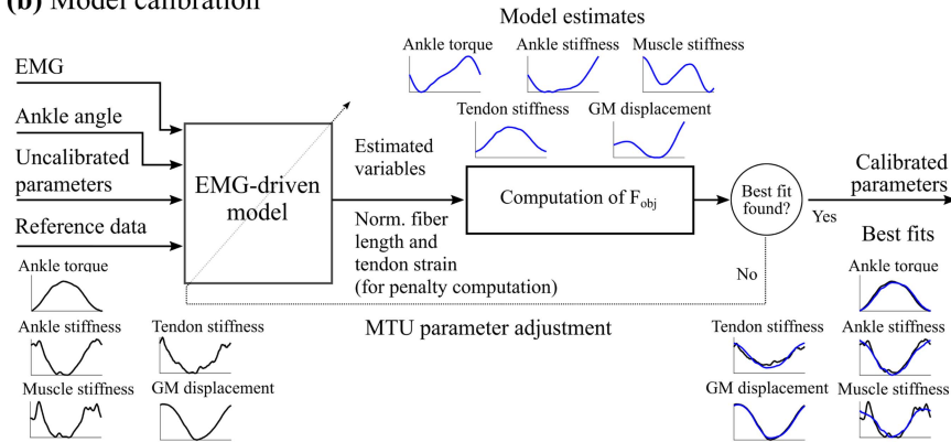
Fig. 3. (a) EMG-driven model: the “Activation dynamics” block maps experimental muscle excitations into muscle-tendon unit (MTU) activations. The “MTU kinematics” block maps ankle plantar-dorsiflexion angle into MTU length. The “MTU dynamics” block estimates MTU force and stiffness employing a Hill-type muscle model driven by MTU activation and length with an elastic tendon. The “Ankle torque and stiffness computation” block projects MTU force and stiffness onto the joint level via the MTU moment arm to obtain estimates of joint torque and stiffness. (b) Model calibration: Seven parameters per MTU, namely optimal fiber length, tendon slack length, maximum isometric force, shape factor, pennation angle at optimal fiber length, stiffness of the tendon force-strain curve and stiffness of the muscle passive force-length curve, are adjusted to best track input reference ankle torque, ankle stiffness, GM displacement, muscle stiffness, and tendon stiffness profiles using the EMG-driven model described in (a). A simulated annealing optimization routine is used to adjust MTU parameters to minimize the difference between reference (plots in black) and estimated (plots in blue) biomechanical variables.
