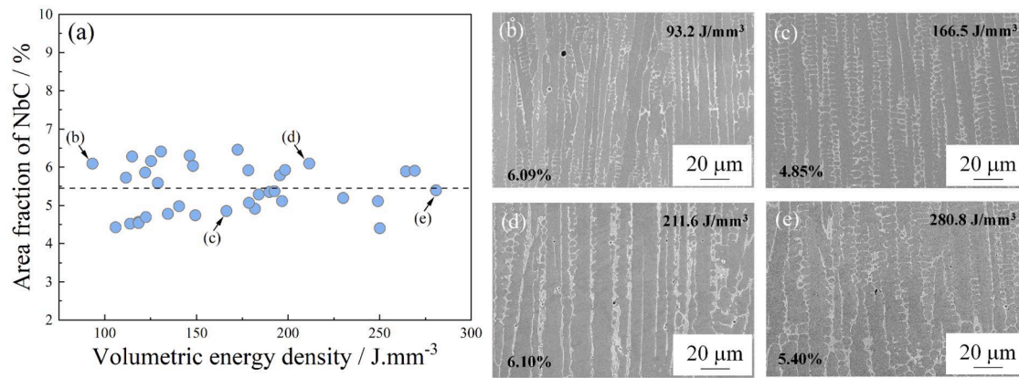
Fig. 13. The area fraction of NbC as a function of volumetric energy density for AMSC-BD alloy (a), and the corresponding representative SEM micrographs (b-e).
