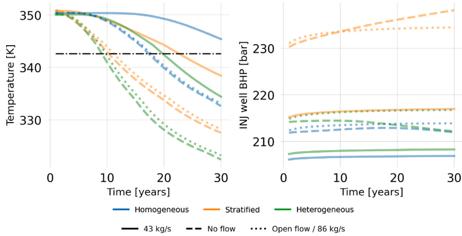
Fig. 15. Temperature and injection well BHP for different types of geological models subject to different geological boundaries: open flow boundary and no flow boundary.
