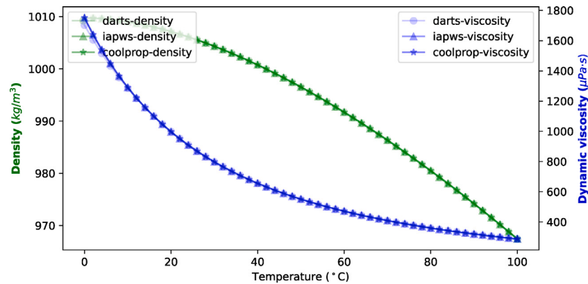
Fig. A.2. The water density and viscosity at the pressure of 200 bar.
