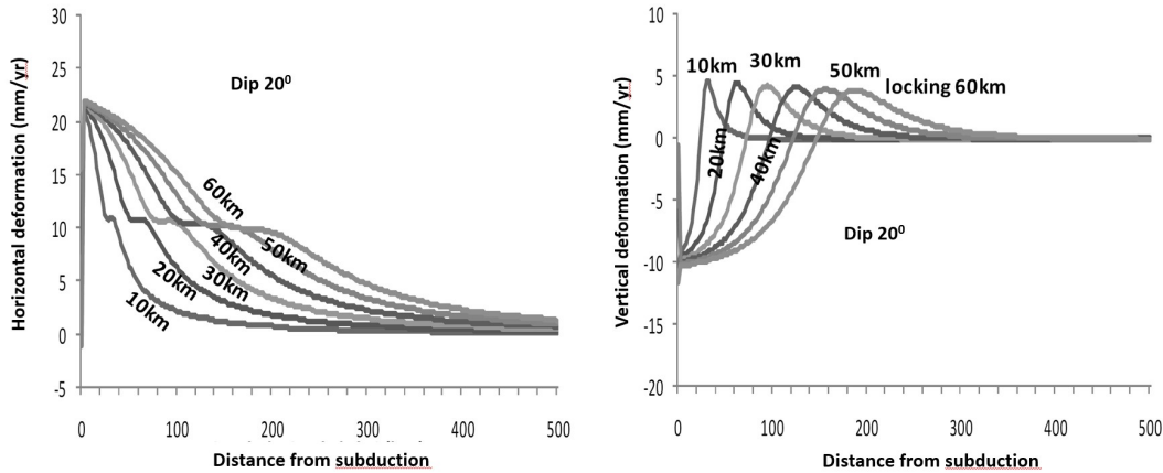
Figure 3. Horizontal (left) and vertical (right) deformation using simple elastic modelling from Okada for subduction zone
