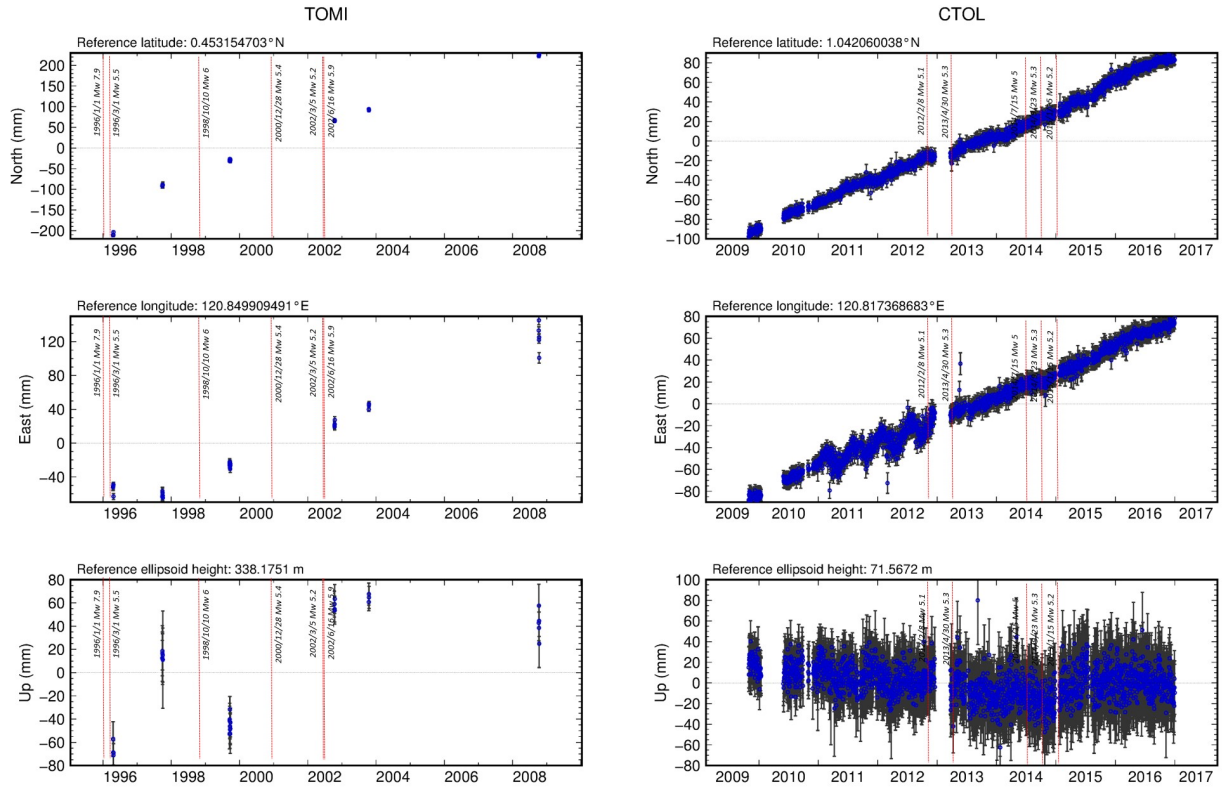
Figure 4. GNSS GPS time series of TOMI station (left) for 1996-2008 analysis and CTOL station (right) for 2009-2016 analysis, with red line as earthquake co seismic event
