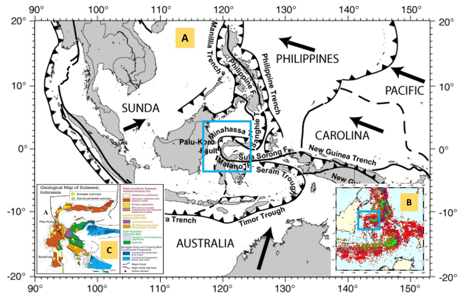
Figure 1. A. Indonesian Tectonics Map [1], B. Earthquake activity from NEIC Catalog and C. Geological Map of Sulawesi [2]
