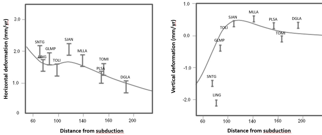
Fig 6. Best-fitting horizontal deformation (left) and vertical (right) with 50 km depth, dip angle 30^\circ and subduction velocity 4 cm/yr
