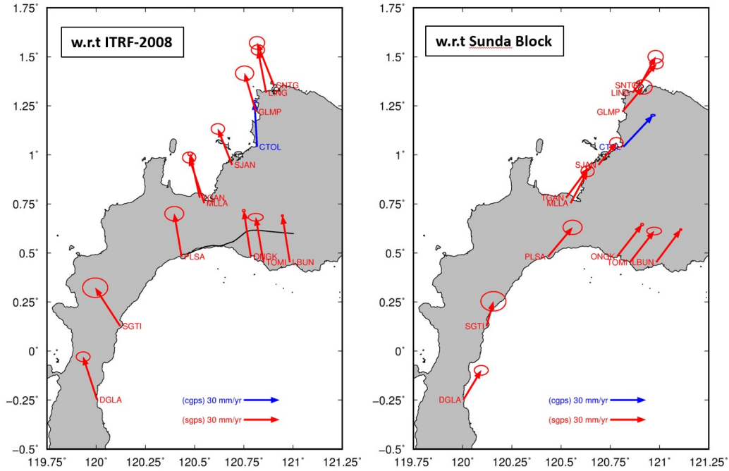
Figure 5. Horizontal velocities of research area w.r.t ITRF 2008 (left) and w.r.t Sunda Block (right)
