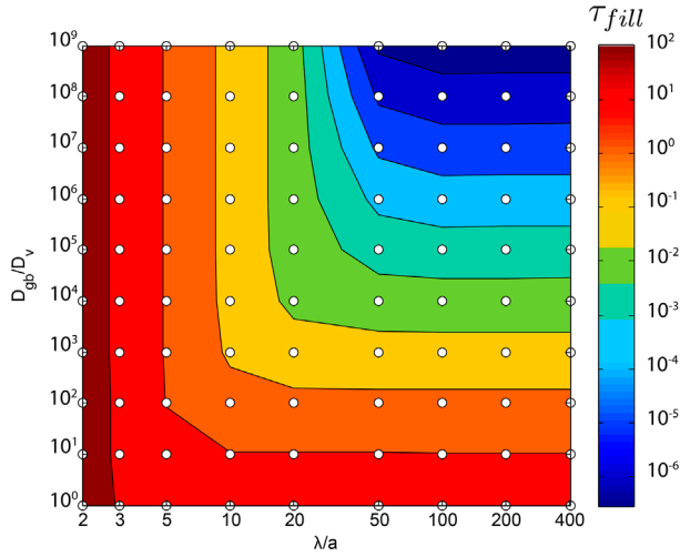
Figure 5. (colour online) Dimensionless filling time \tau_{fill} as a function of \lambda/a and D_{gb}/D_V . All data are for a supersaturation of \Delta c = 0.01 .
