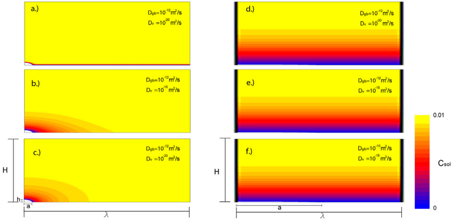
Figure 2. (colour online) Solute concentration around the cavity at the time of filling. (a) \lambda/a = 20 , and D_{gb}/D_V = 10^8 . (b) \lambda/a = 20 , and D_{gb}/D_V = 10^3 . (c) \lambda/a = 20 , and D_{gb}/D_V = 1 . (d) \lambda/a = 2 , and D_{gb}/D_V = 10^8 . (e) \lambda/a = 2 , and D_{gb}/D_V = 10^3 . (f) \lambda/a = 2 , and D_{gb}/D_V = 1 . All data are for a supersaturation of \Delta c = 0.01 . For \lambda/a = 2 , the grain boundary contains insufficient solute, and as a result, a quasi-1D profile is observed at the time of filling, independent of the ratio D_{gb}/D_V .
