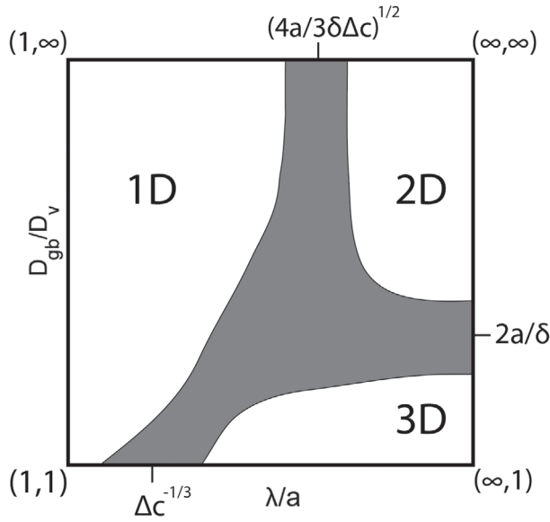
Figure 7. Phase diagram for the diffusional character of creep cavity filling by supersaturated solute, as a function of the diffusivity ratio D_{gb}/D_v and the characteristic length scale ratio \lambda/a . 3 different regimes with 1D, 2D and 3D diffusion are observed. The characteristic values for the cross-over between these regimes are indicated.
