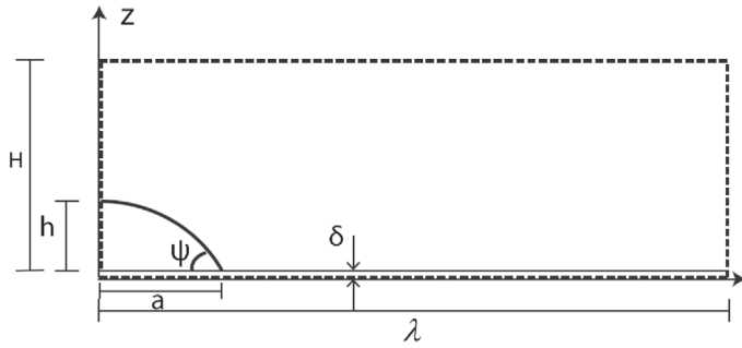
Figure 1. Lens-shaped creep cavity defined by an opening angle \psi , a height h and a radius a . The creep cavity is formed on a grain boundary with width \delta . The simulation box is a cylinder with a radius \lambda and a height H .
