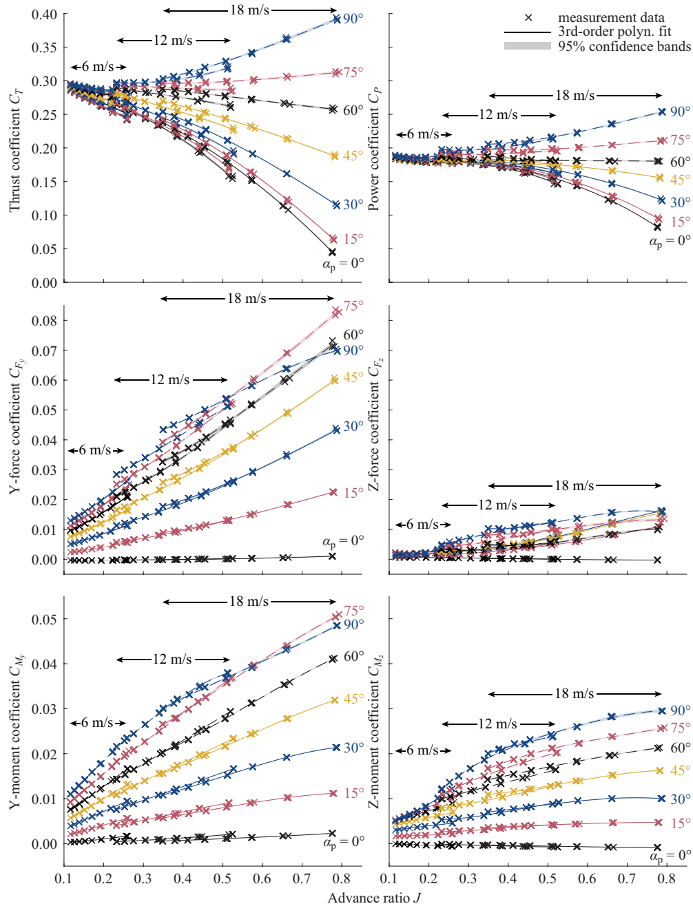
Fig. 12 Experimental result showing thrust, power, in-plane force, and out-of-plane moment coefficients for \beta_{0.7R_p} = 20^\circ deg.
