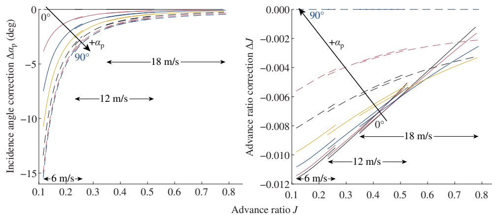
Fig. 13 Angle of attack and advance ratio wind tunnel wall corrections for the experimental results for \beta_{0.7R_p} = 20^\circ deg; line style and color of Fig. 12 maintained.
