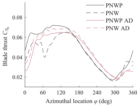
Fig. 26 CFD blade thrust evolution showing effect of pylon and nonuniform actuator-disk modeling ( \beta_{0.7R_p} = 20 deg, J = 0.35 , V_{\infty} = 18 m/s, d_w/R_p = 0.4 , and \delta_f = 0 deg); azimuthal location \varphi is defined in Fig. 19.
