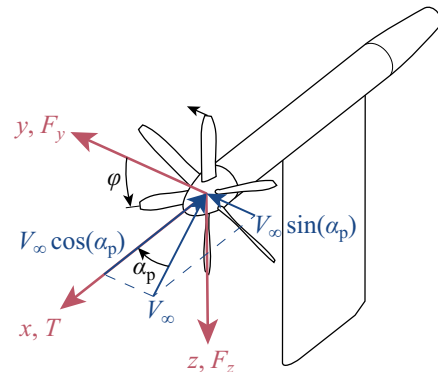
Fig. 7 Sketch of propeller setup without wing, including definition of propeller reference frame, blade phase angle \phi , angle of attack \alpha_p , free-stream velocity components, and force components.
