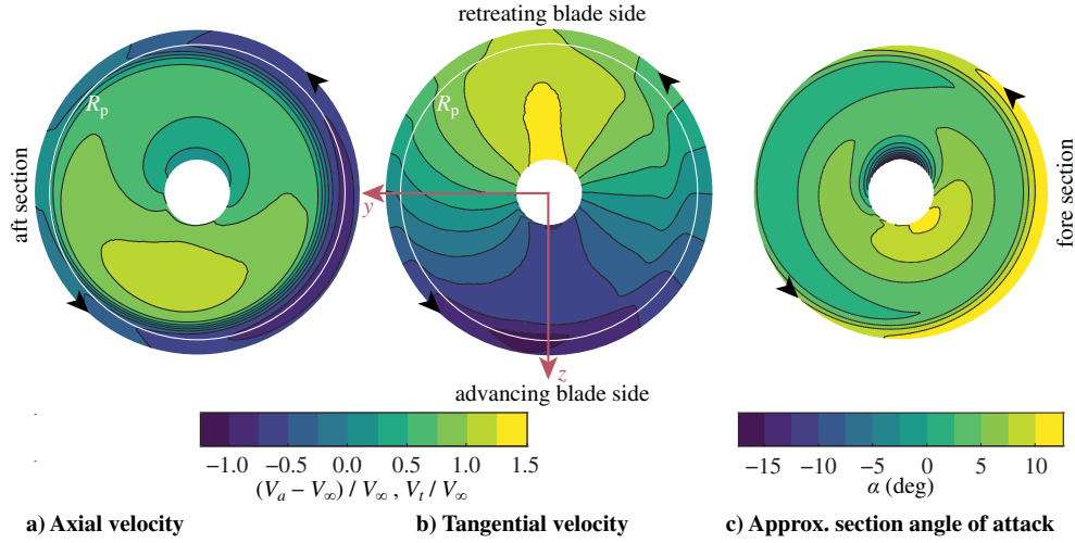
Fig. 17 CFD PN result showing time-averaged propeller flowfield at \alpha_p = 45^\circ ( \beta_{0.7R_p} = 20^\circ , J = 0.35 , and V_\infty = 18 m/s).
