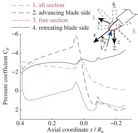
Fig. 18 CFD PN result showing the time-averaged C_p distribution on the spinner in a horizontal and vertical plane at \alpha_p = 45^\circ ( \beta_{0.7R_p} = 20^\circ , J = 0.35 , and V_\infty = 18 m/s).
