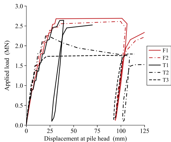
Fig. 7. Load–displacement response under axial compressive loading.
