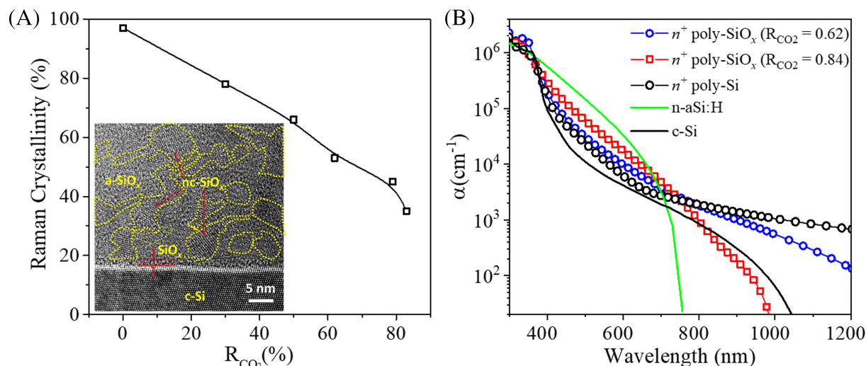
FIGURE 2 (A) The Raman crystallinity as a function of gas ratio, R_{CO_2} = [\text{CO}_2]/([\text{CO}_2]/[\text{SiH}_4]) , for n^+ poly-SiO x samples, which were deposited on quartz glass and underwent annealing at 850°C for 30 min. The inset is a transmission electron microscopy (TEM) picture measured on sample with R_{CO_2} = 0.62 at the poly-SiO x /NAOS-SiO x /c-Si interfaces. (B) The absorption coefficient ( \alpha ) curves of n^+ poly-Si samples with R_{CO_2} = 0.62 and 0.84 as a function of wavelength; the \alpha curves related to n^+ poly-Si, 47 a-Si:H, 48 and c-Si (n) 49 are used as references
