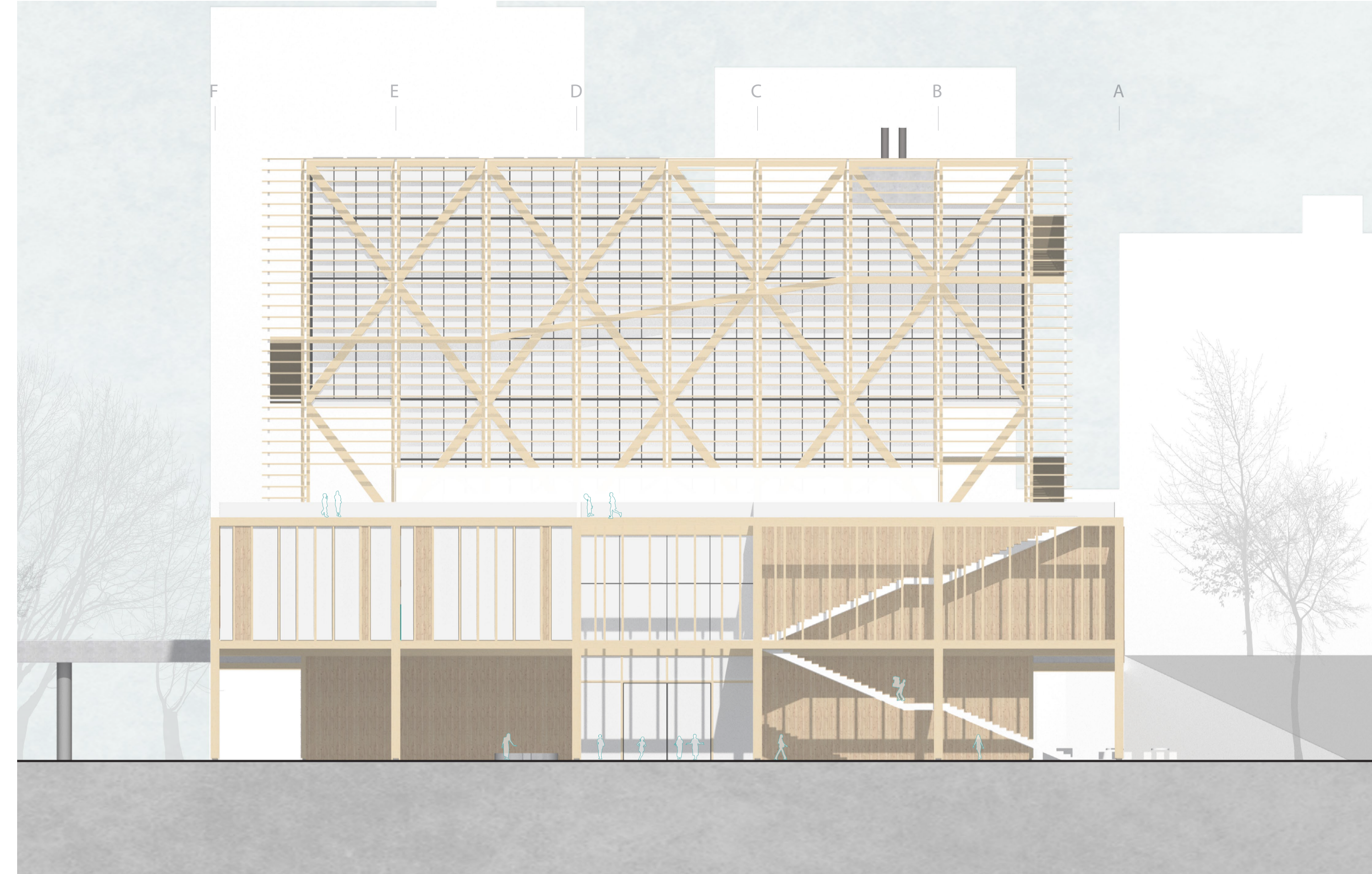
FACADE WEST
