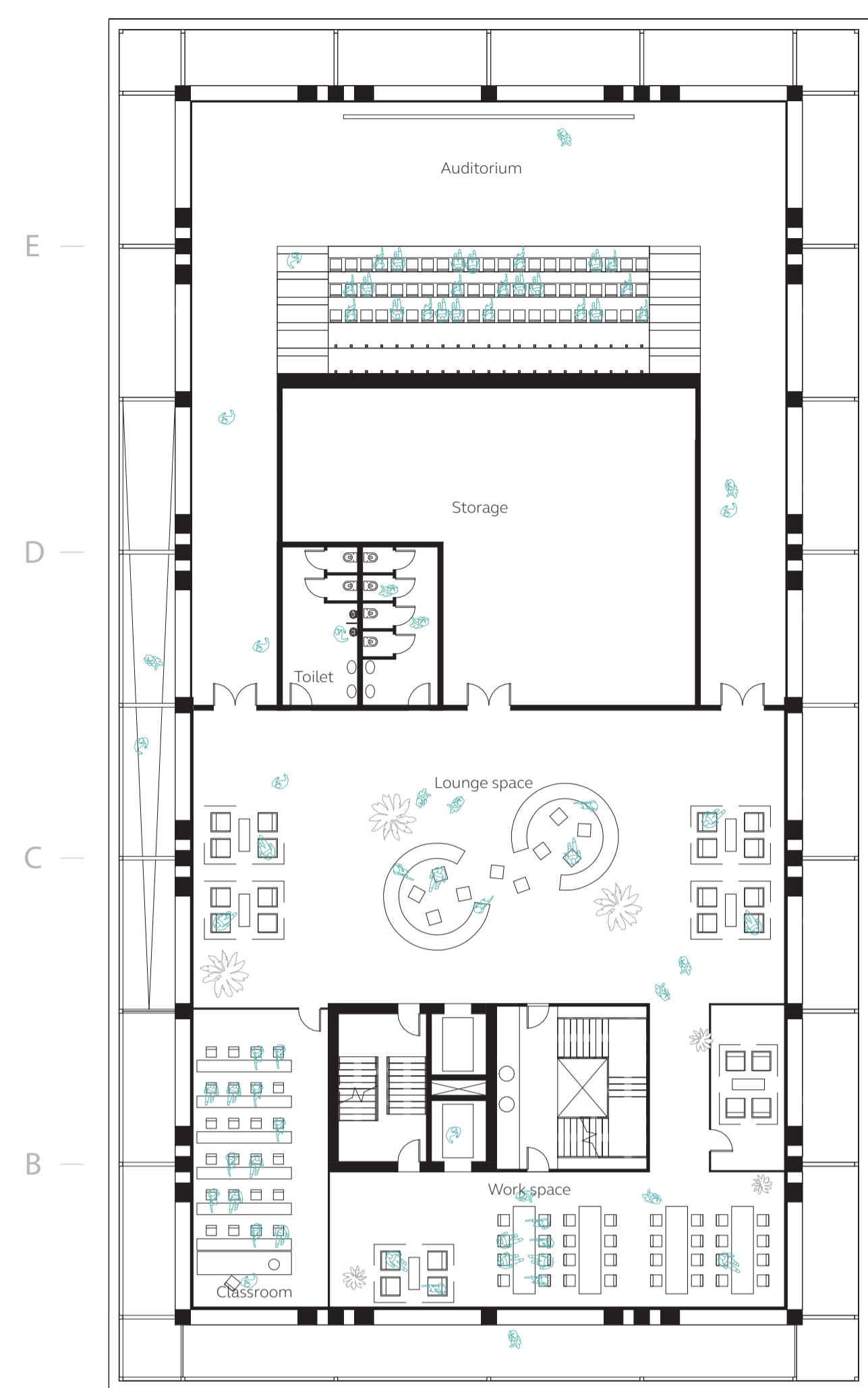
SEVENTH FLOOR
