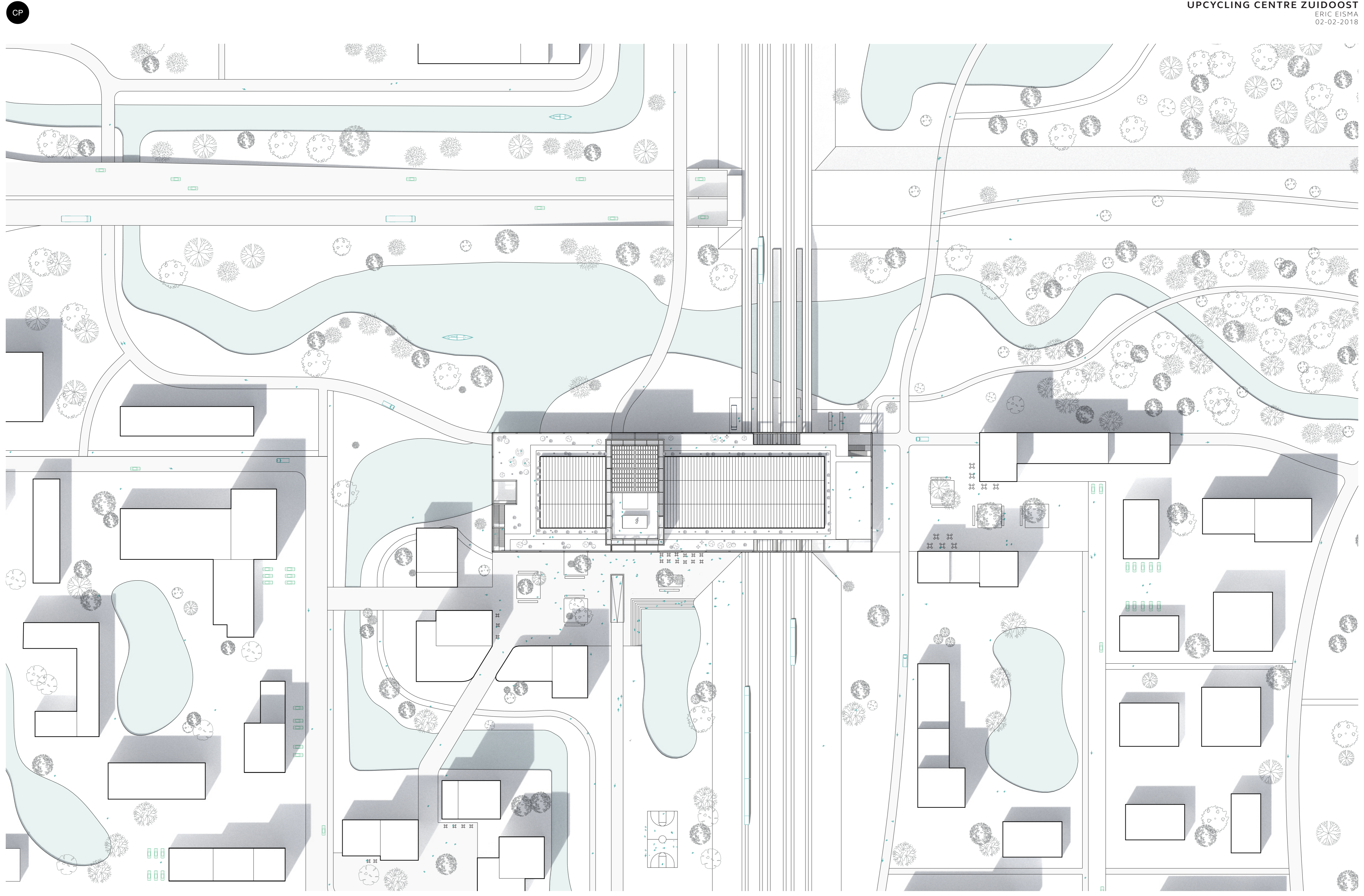
10m 20m 50m 100m SITE ROOF PLAN 1:1000
