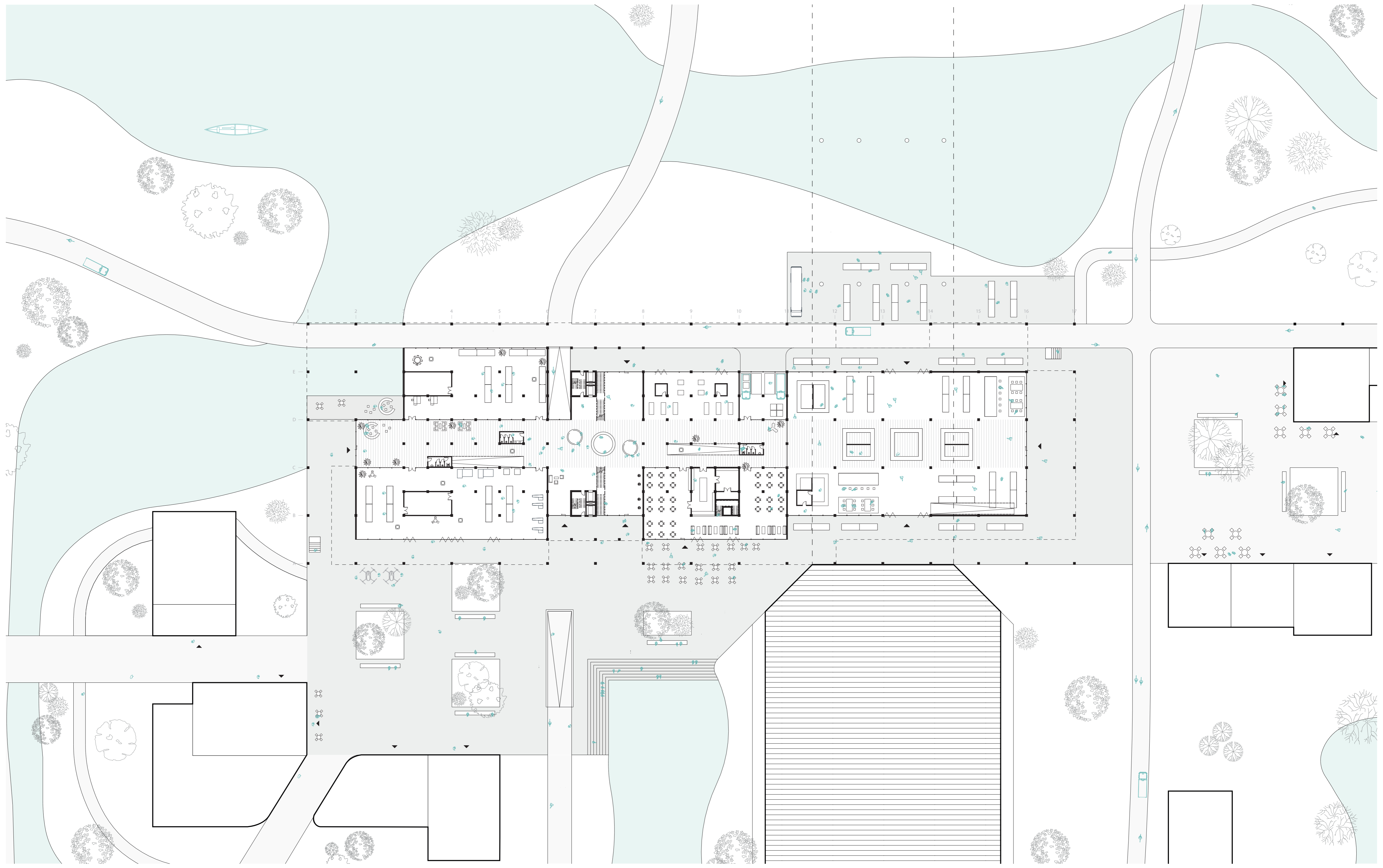
5m 10m 25m 50m URBAN IMPLEMENTATION 1:500
