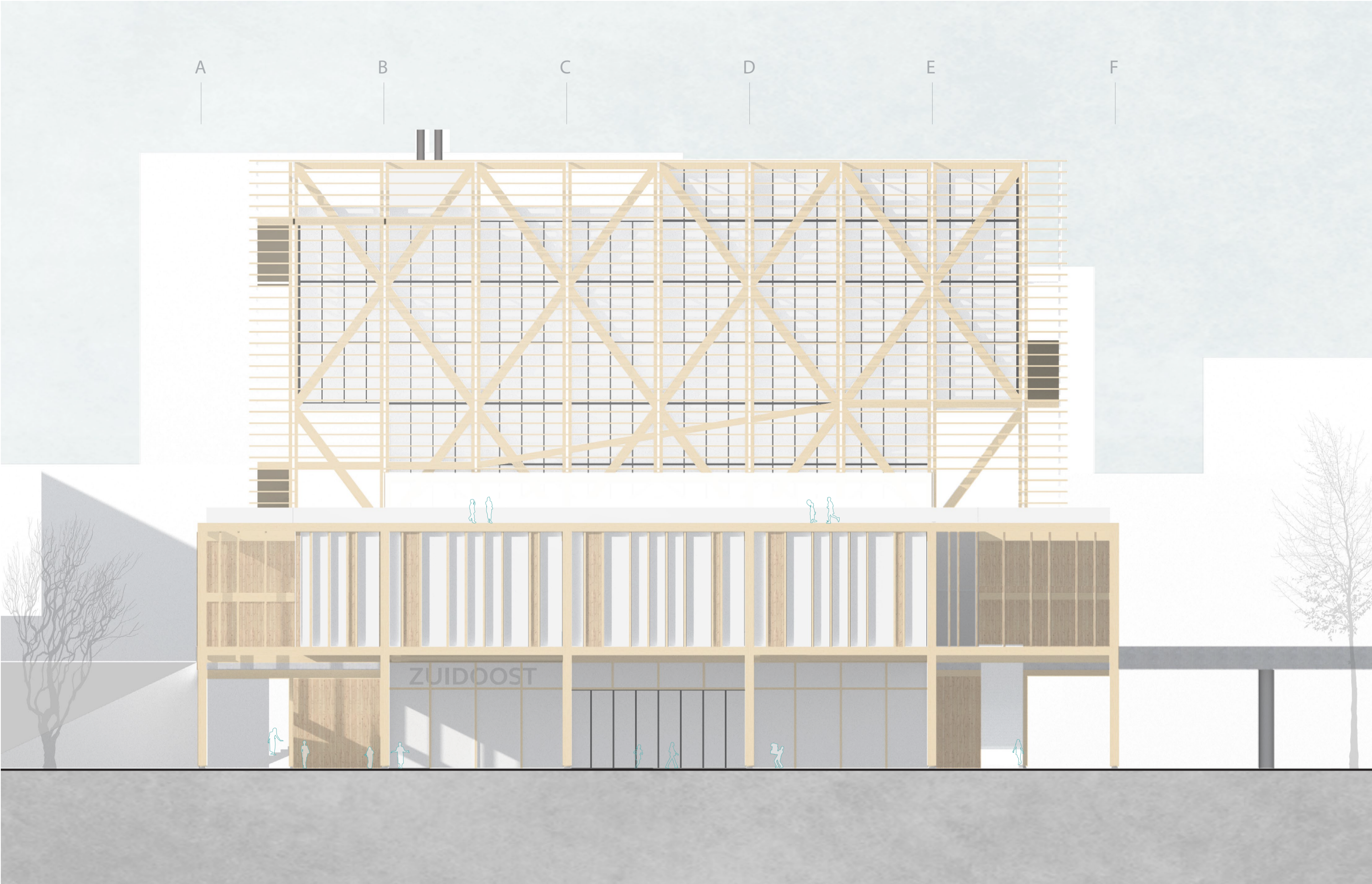
FACADE EAST
