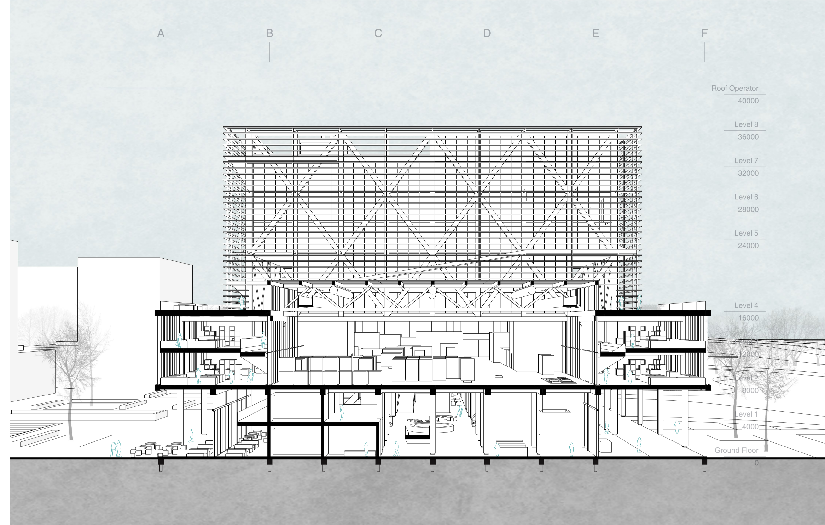
SECTION CC
