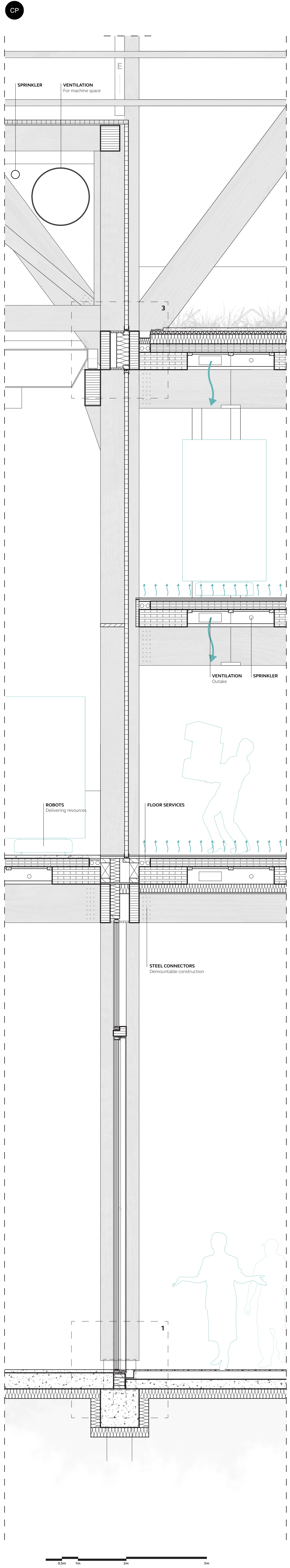
DETAIL SECTION CC 1:25
