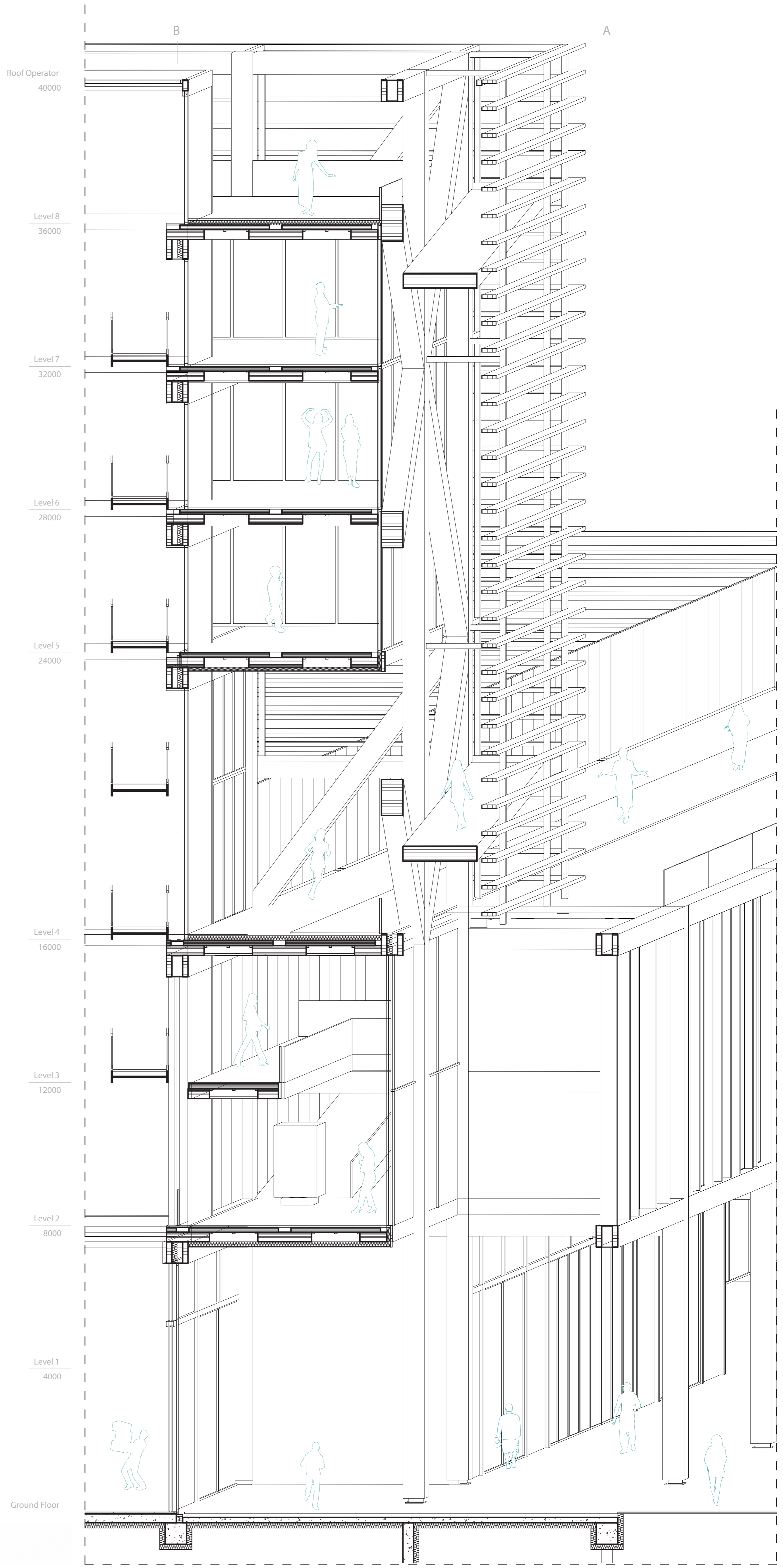
SECTION BB
