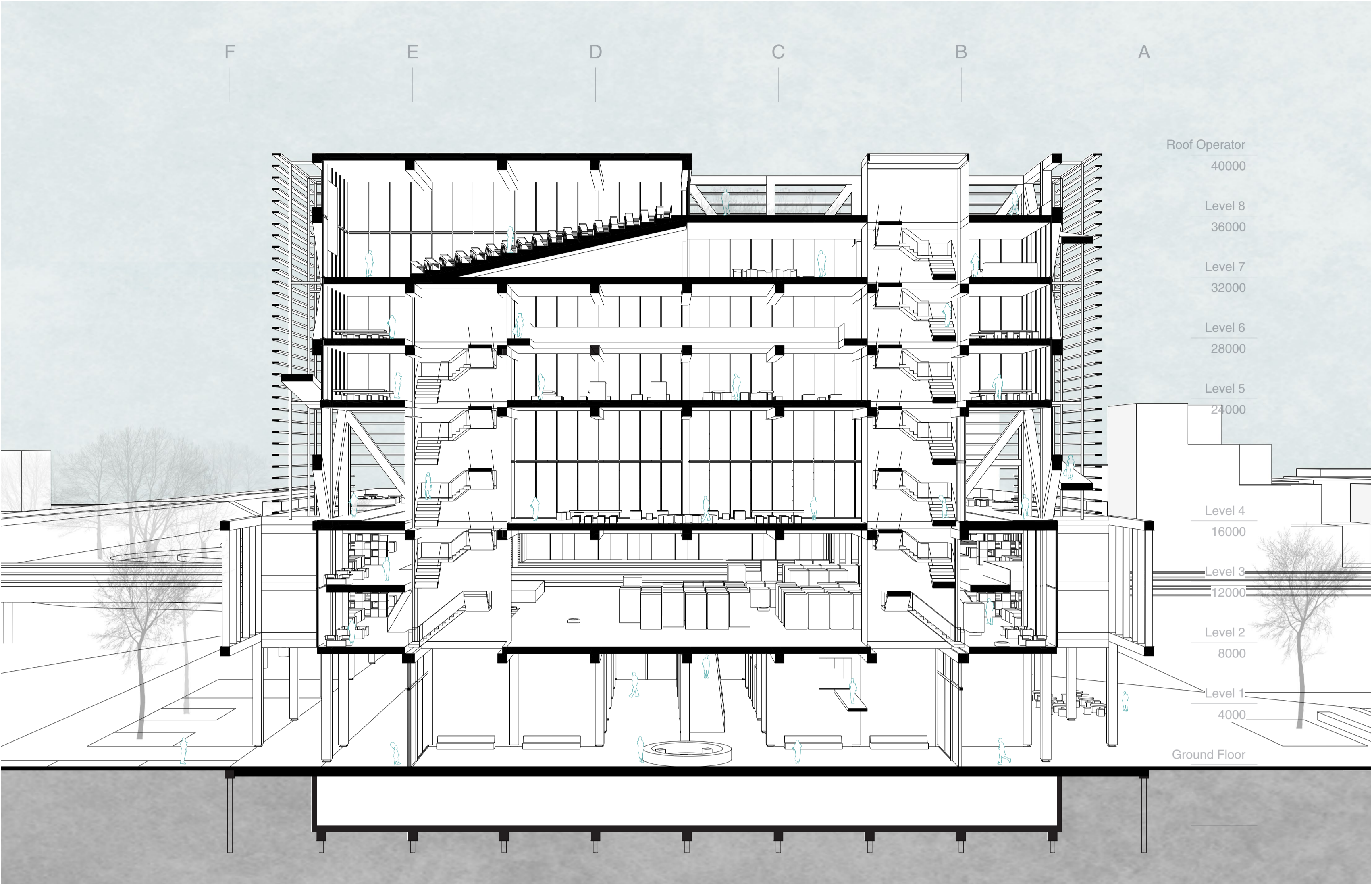
SECTION BB
