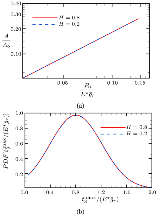
Fig. 8. (a) Relative contact-area a_r versus normalized nominal-pressure P_0/(E^* \bar{g}_r) for different Hurst exponents. (b) Probability density function of the traction peaks \text{PDF}[t_3^{lmax}/(E^* \bar{g}_r)] .
