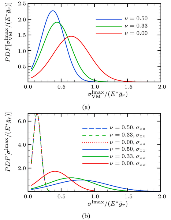
Fig. 13. Effect of Poisson's ratio on the probability density function of a) \sigma_{VM}^{\text{max}} b) \sigma_{xx}^{\text{max}} and \sigma_{xz}^{\text{max}} .
