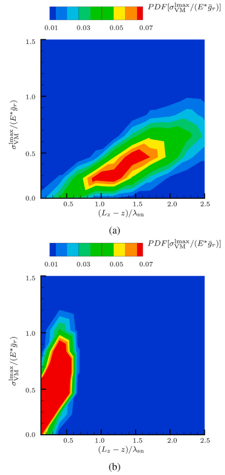
Fig. 18. Distributions of \sigma_{VM}^{max} / (E^* \bar{g}_r) along the depth of the body for surfaces with kurtosis (a) G(\mathbf{r}) : \lambda_s = L_x/128 and (b) K_2(\mathbf{r}) : \lambda_s = L_x/512 . \lambda_{sn} = L_x/128 .
