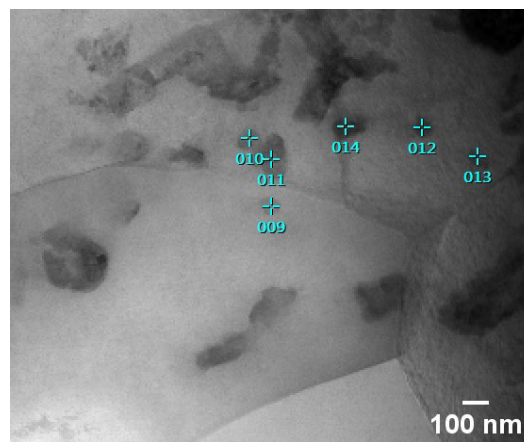
Fig. 3. TEM bright field image of extruded nanocompositions containing TiN nano powder.
