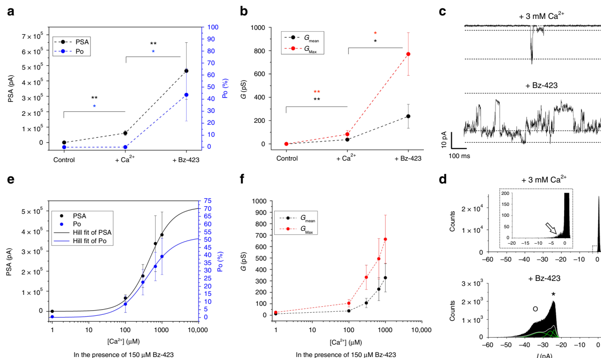
Fig. 5 \text{Ca}^{2+} -dependence and activation of F-ATP synthase channels by Bz-423. a Power spectrum area (PSA) and open probability ( P_o ) of F-ATP synthase channels were calculated from five independent experiments in the absence of activators (control), after addition of 3 mM \text{Ca}^{2+} alone or following the addition of both 3 mM \text{Ca}^{2+} and 0.15 mM Bz-423. Zero values are indicated with black and blue dotted lines for PSA and P_o , respectively. Data shown are mean \pm SEM. Statistical significance of differences was assessed with the Mann-Whitney test (* p \leq 0.05 , ** p \leq 0.01 ). b Mean and maximal conductance ( G_{\text{mean}} and G_{\text{max}} ) were calculated for the same experiments shown in panel a . c Current traces elicited after addition of 3 mM \text{Ca}^{2+} alone or after further addition of 0.15 mM Bz-423 ( V_{\text{cis}} = -60 mV, G_{\text{max}} = 500 pS) from one representative experiment of five. The closed state is denoted with C, the most frequent subconductance state with an asterisk, and the maximal open state with O. d Current distribution of 30 s-recordings from experiments similar to the one reported in panel c . In the presence of \text{Ca}^{2+} alone, flickering openings may be observed as a small peak in the histogram (arrow), while in the presence of Bz-423, a complex distribution with multiple peaks at higher conductance values (400 and 500 pS) is detectable. e PSA and P_o of F-ATP synthase channels as a function of the \text{Ca}^{2+} concentration in the presence of 0.15 mM Bz-423; PSA and P_o distributions were fitted with the Hill equation ( n = 1.37 \pm 0.29 , R^2 = 0.992 ; n = 1.17 \pm 0.16 , R^2 = 0.997 , respectively). Data were obtained from 23 independent experiments and are shown as mean \pm SEM. f G_{\text{mean}} and G_{\text{max}} of F-ATP synthase channels as a function of the \text{Ca}^{2+} concentration from the same experiments shown in panel e . The source data underlying panels a , b , e , f are provided as a Source Data file
