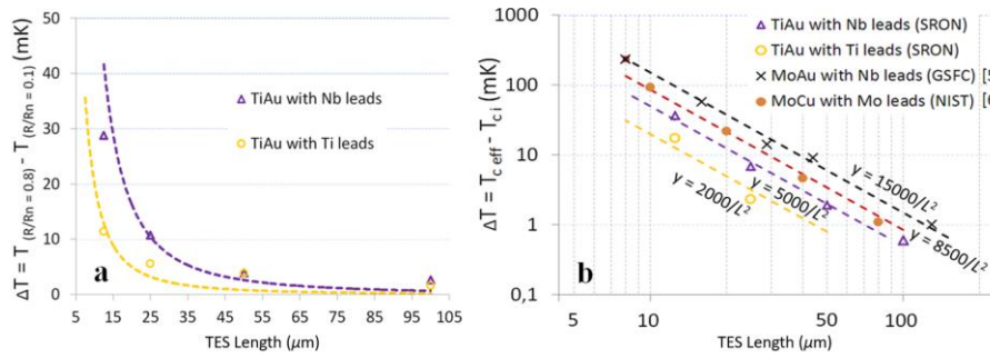
Fig. 5 The graph on the left (a) shows the width of the transition curve defined as \Delta T = T_{(R/RN = 0.8)} - T_{(R/RN = 0.1)} versus TES length. On the right side (b) the \Delta T = T_{ceff} - T_{ci} is plotted as a function of the TES lengths.
