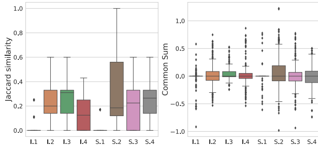
Figure 7: Coherence - Left: Results from Equation 6, Right: Results from Equation 7. The x-axis labels represent different configurations; (I) Inception V3, and (S) SqueezeNet; Biases: (1) Negative Set Bias, (2) No Bias (Utensils), (3) Colour (Utensils), (4) Shape (Utensils).
