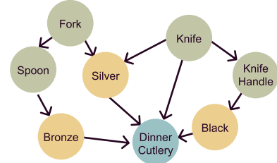
Figure 3: Causal Graph example, including primary concepts (green), mediating concepts (yellow), and the model outcome (blue) for the “Dinner Cutlery” class.
