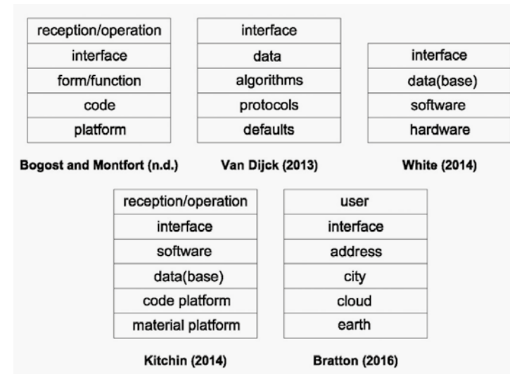
Fig. 1 Examples of 'digital technology stack' concepts from literature. Diagram adapted from Rob Kitchin, 'From a Single Line of Code to an Entire City: Reframing the Conceptual Terrain of Code/Space', in: Rob Kitchin and Sung-Yueh Perring (eds.), Code and the City (Abingdon, Oxon: Routledge, 2016), 20.
