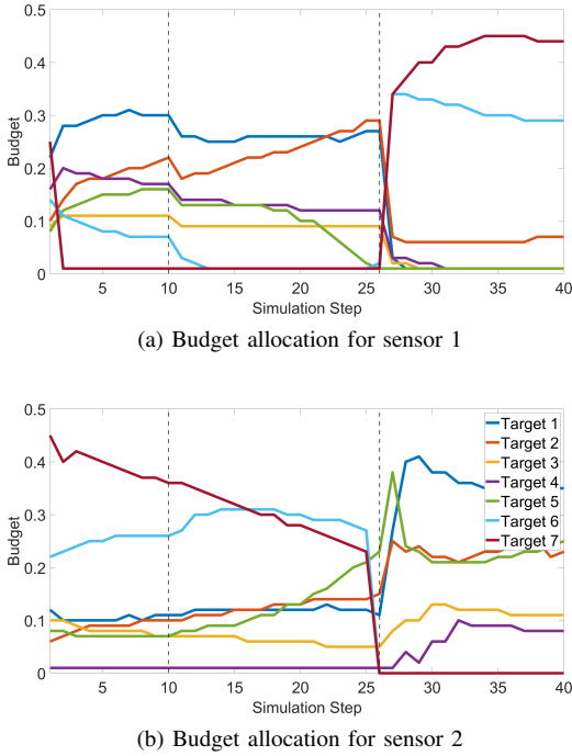
Fig. 4. Budget allocations over multiple simulation steps. At time step k = 10 the maximum budget for sensor 1 is reduced to 0.8. At time step k = 26 sensor 2 can no longer track targets 6 and 7.
