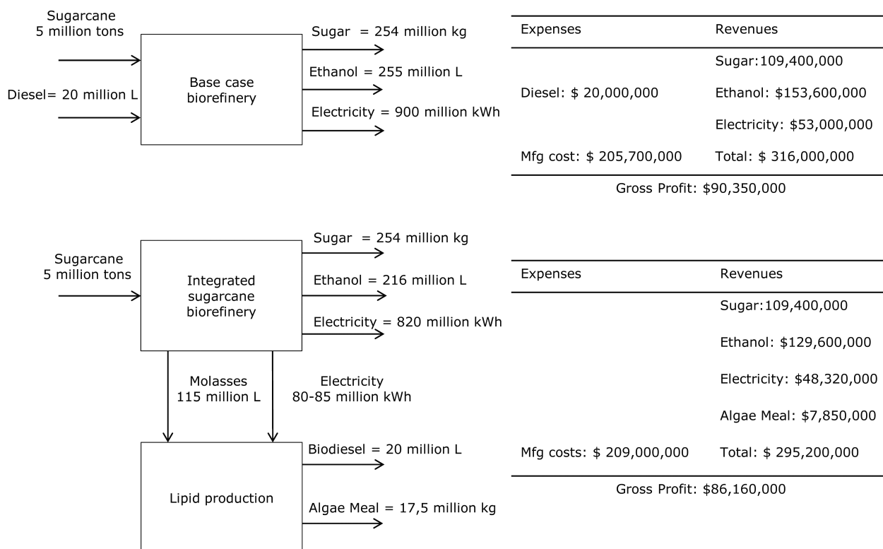
Figure 5. Inputs and outputs and profitability comparison between the base case sugarcane refinery and the integrated microalgae-sugarcane refinery.
