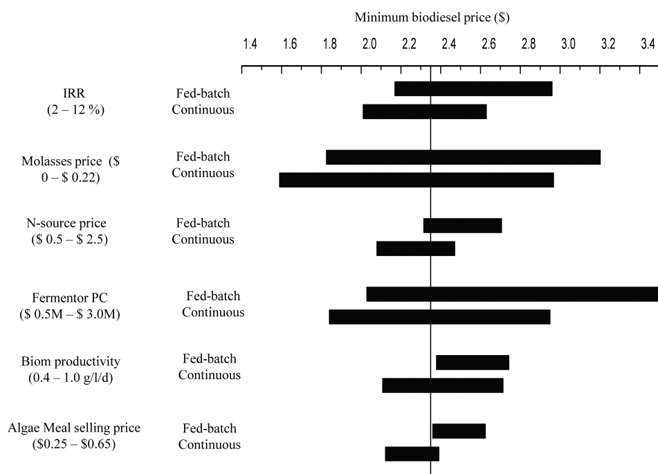
Figure 4. Sensitivity analysis of minimum biodiesel selling price for an independent (non-integrated) microalgae plant against the most important cost factors.
