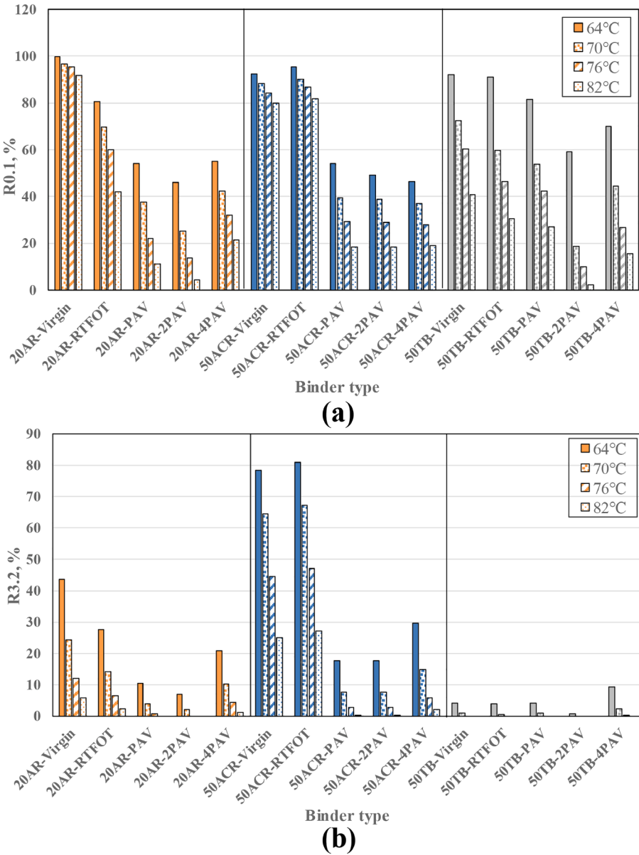
Fig. 12. R of 20AR, 50ACR, and 50 TB before and after aging: (a) R0.1; (b) R3.2.
