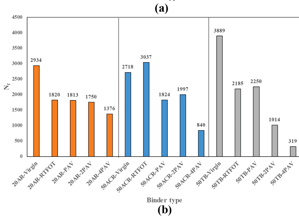
Fig. 17. N_f at different strain levels: (a) N_f of 20AR, 50ACR, and 50 TB at 2.5% strain, (b) N_f of 20AR, 50ACR, and 50 TB at 5% strain.
