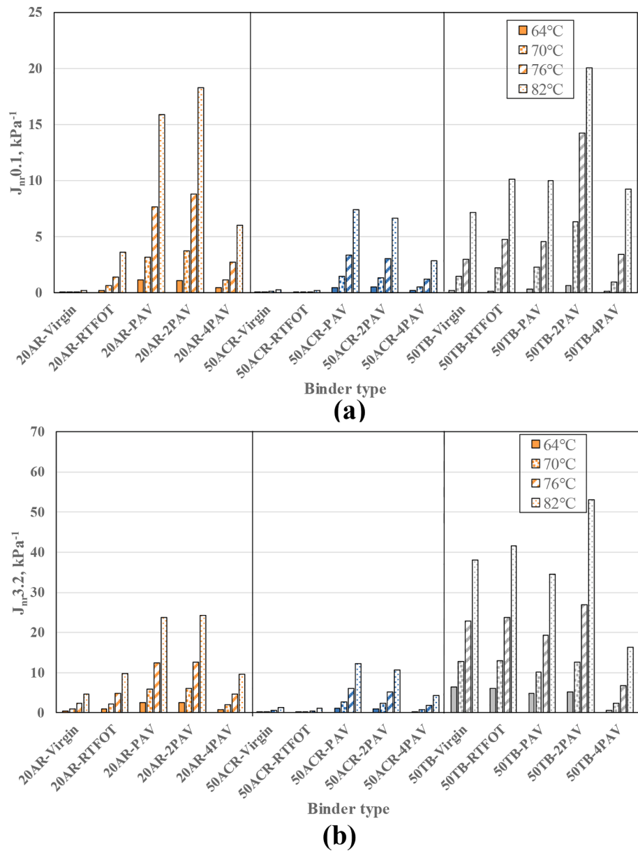
Fig. 11. J_{nr} of 20AR, 50ACR, and 50 TB before and after aging: (a) J_{nr,0.1} ; (b) J_{nr,3.2} .
