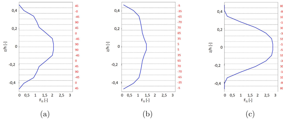
Fig. 3. Through the thickness distribution of f_{1s} in several laminates: (a) reference laminate, [45/0/-45/90] 2s , ( \max(f_{1s}) = 2.05 ); (b) best optimum dispersed-ply laminate, B1: [-5/-35/-65/-70/70/65/35/5] s , ( \max(f_{1s}) = 1.47 ); (c) non-optimal dispersed-ply laminate with lower performance than the reference, [80/-80/10/-10/30/-30/55/-55] s , ( \max(f_{1s}) = 2.89 ).
