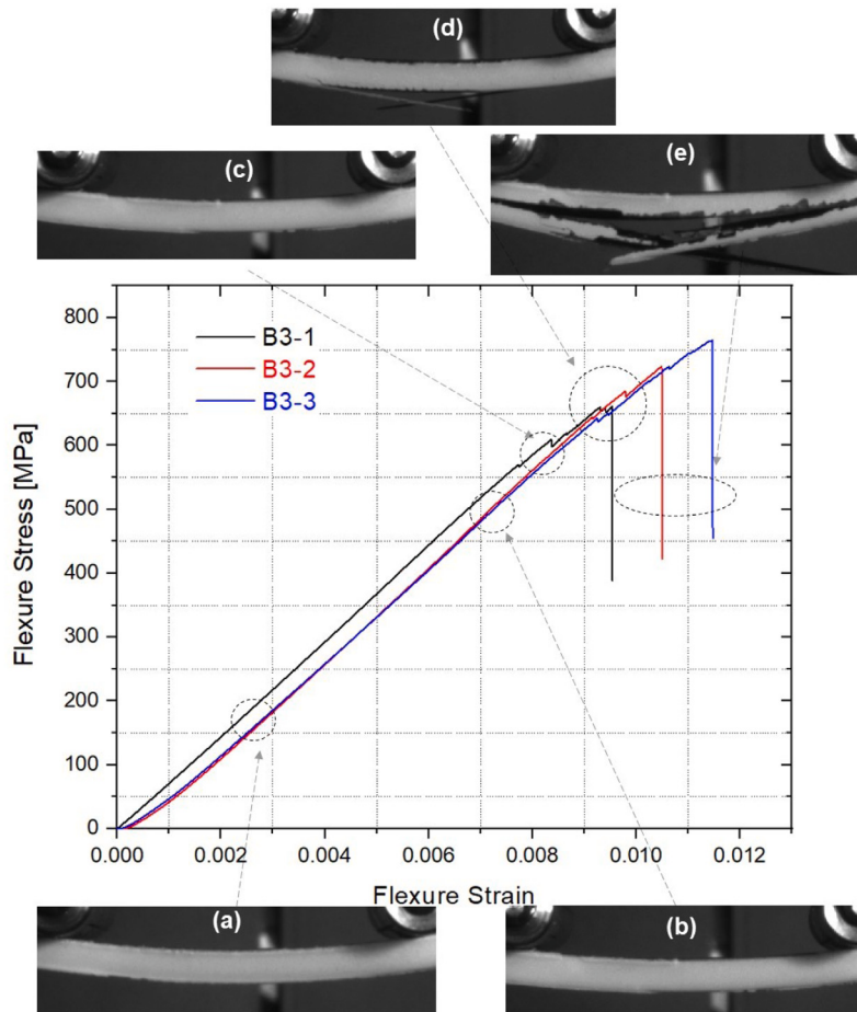
Fig. 7. Four-point bending test for “B3” laminate [-5/-45/-45/90/90/45/45/5]_1 .
