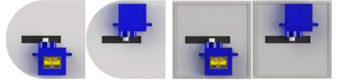
Fig. 4. Constrained by the locations of slits, each SG90 servomotor c_{SG_i} can only have two candidate locations \{\Theta_{SG_i,1}, \Theta_{SG_i,2}\} (above or below the slit) on one of the three faces with slits in the male box.
