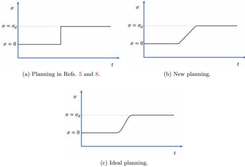
Figure 3: Options for bank-angle planning for Phase 1.
