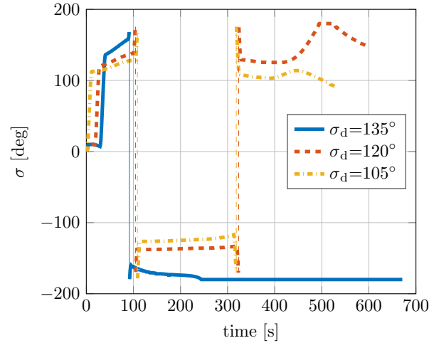
Figure 10: Bank angle history for OAK guidance with different values of \sigma_d , in a case of strong perturbations.
