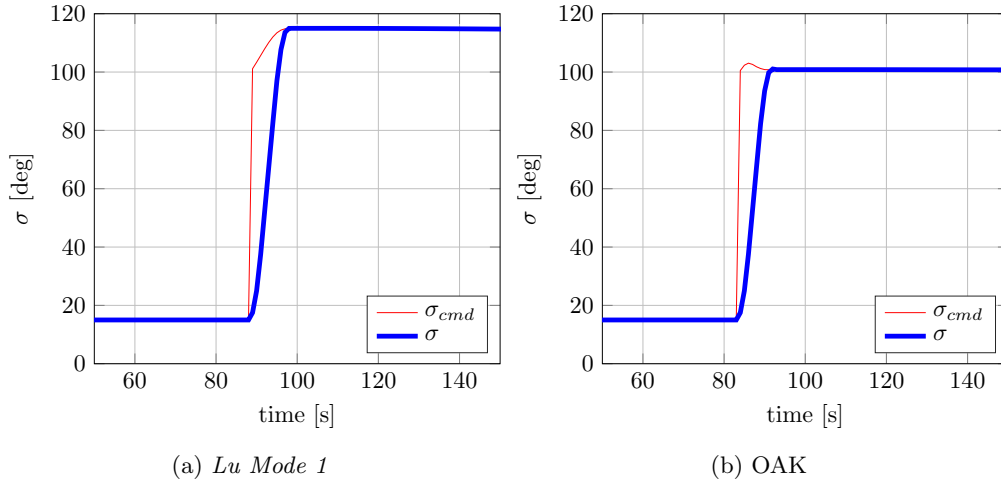
Figure 6: Bank-angle history during flight in ideal conditions, \sigma_d = 100^\circ .
