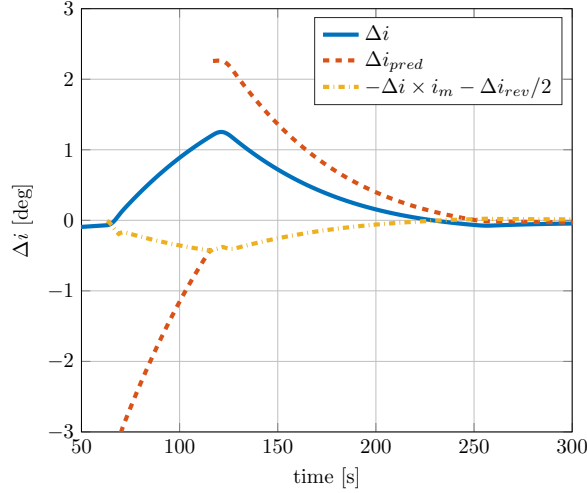
Figure 4: Schematic of the lateral logic during Phase 2; i_m = 0.3 .
