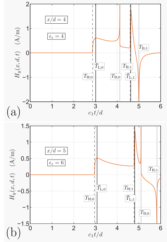
Fig. 8. Unit-step-excited magnetic-field strength at (a) (x, z) = (4d, d) for \epsilon_r = 4 and (b) (x, z) = (5d, d) for \epsilon_r = 6 .
