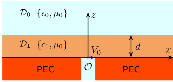
Fig. 6. Slot-excited dielectric slab.
