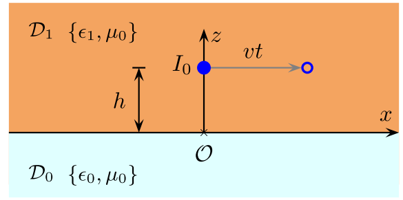
Fig. 1. Impulsive electric-line source above a half-space.
