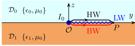
Fig. 11. Ray trajectories of the HW, LW, and BW constituents around the interface. The LW trajectory is represented by the blue wavy line.
