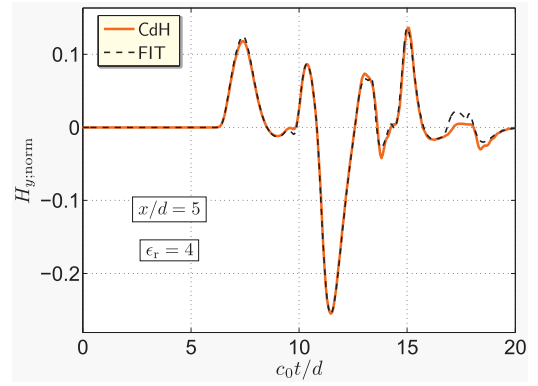
Fig. 12. Magnetic-field strength [normalized with respect to (\epsilon_0/\mu_0)^{1/2} V_{\max}/w ] at x/d = 5 on the slot-excited dielectric slab of relative permittivity \epsilon_r = 4 as calculated analytically using the CdH technique and numerically using the FIT.
