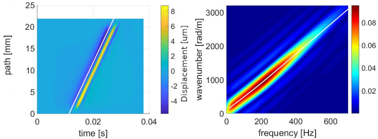
Figure 2: Wave propagation recorded on a 2.2 cm long m-line in a 4 cm long, 9 mm thick flat plate, at a depth of 0.9 mm. On the left image the wave is represented in the x-t domain, and the white line shows a Radon Sum estimation of the trajectory of the wave. On the right image, the wave is represented in the f-k domain, and the white line represents the theoretical A0 dispersion curve for a plate in water with the same geometry and medium properties. The color scheme represents the magnitude of the Fourier-transformed displacement recorded along the m-line.
