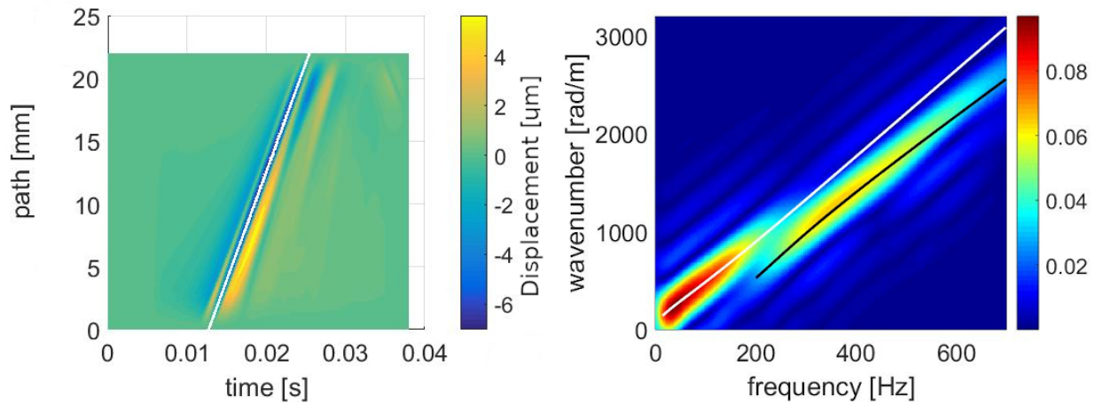
Figure 3: Wave propagation recorded on a 2.2 cm long m-line in a 4 cm long, 9 mm thick flat plate, at a depth of 4.5 mm. On the left image the wave is represented in the x-t domain, and the white line shows a Radon Sum estimation of the trajectory of the wave. On the right image, the wave is represented in the f-k domain, and the white and black lines represents, respectively, the A0 and A1 theoretical dispersion curves for a plate in water with the same geometry and medium properties. The color scheme represents the magnitude of the Fourier-transformed displacement recorded along the m-line.
