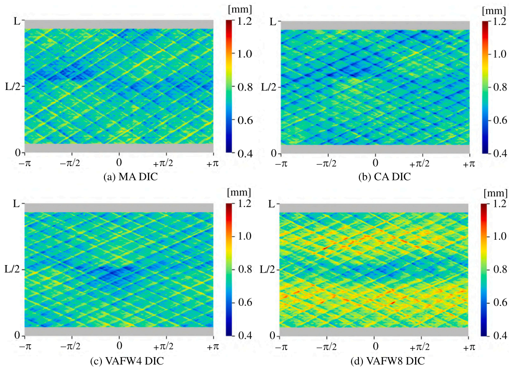
Fig. 8. Experimentally-measured geometric (thickness) imperfection patterns [32]. The gray areas represent the edges with resin potting. (For interpretation of the references to color in this figure legend, the reader is referred to the web version of this article.)
