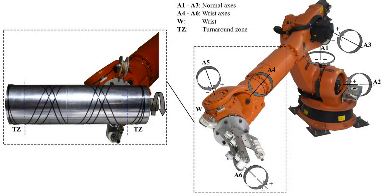
Fig. 4. The used Kuka robot and photograph of a VAFW8 cylinder being manufactured.
