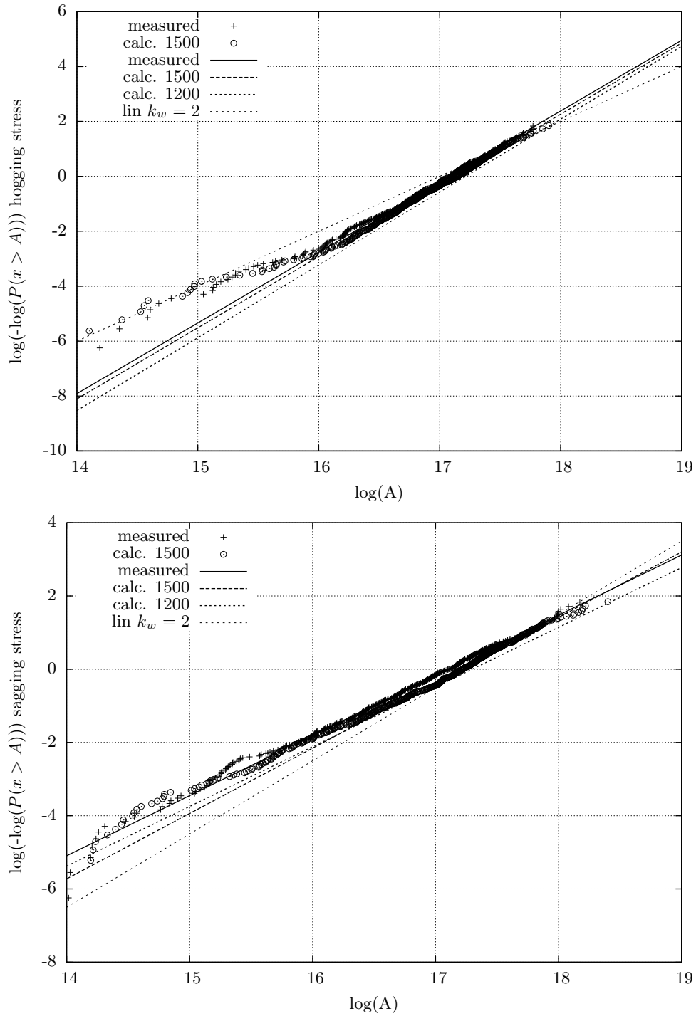
Figure 12.17: Weibull plots for 12 knots including whipping response.
