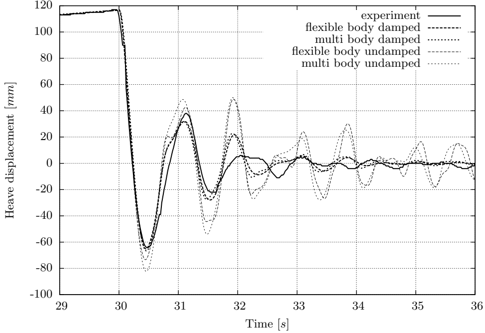
Figure 9.11: Heave displacement of the first floater during decay test.
