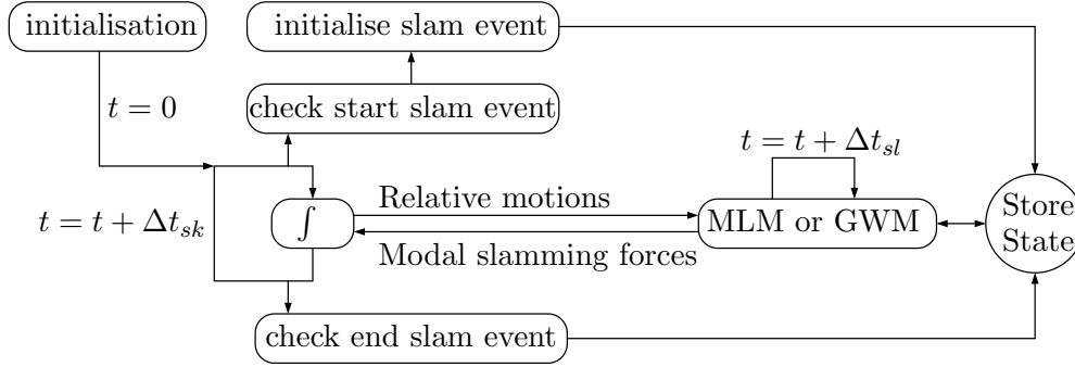
Figure 5.9: Approach for coupling between the seakeeping and the slamming calculations.
