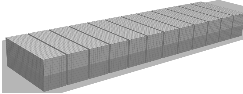
Figure 9.9: Multi-body mesh for time domain calculation.
