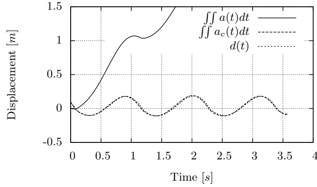
Figure 10.7: Displacements at accelerometer number 1.
