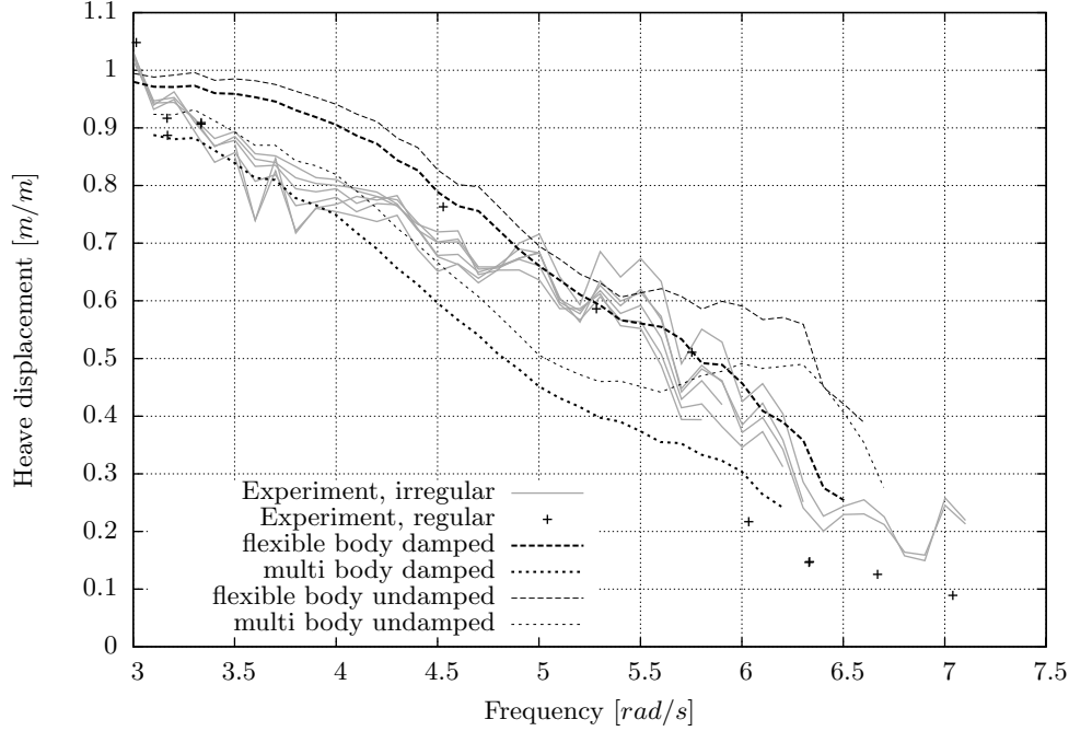
Figure 9.13: RAO heave of the seventh floater.
