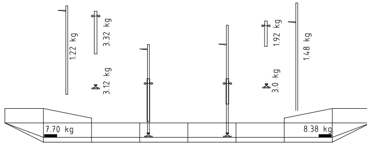
Figure D.1: Mass of additional components.
