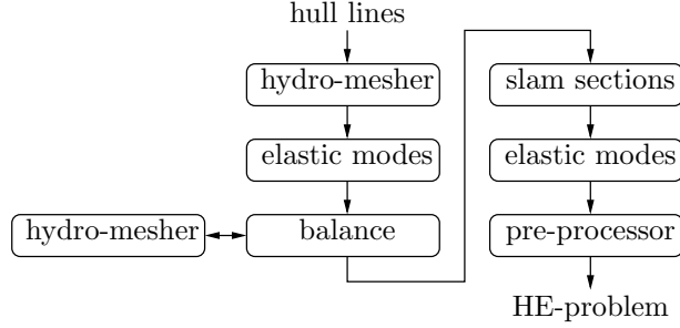
Figure 2.4: Creating input for a balanced flexible body with slamming sections.
