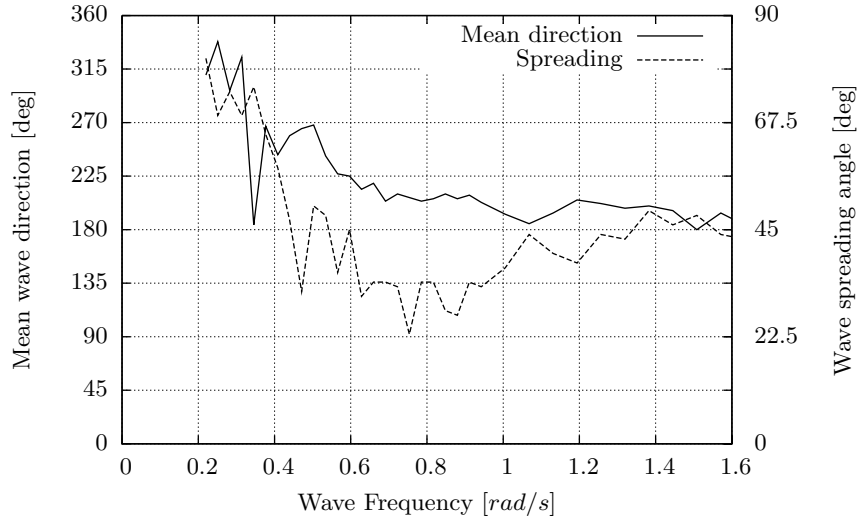
Figure 12.13: Spreading of the 09:00 hour waves.
