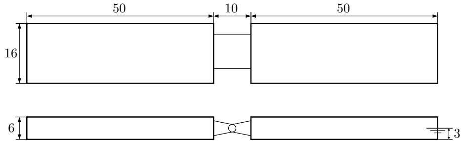
Figure 9.1: Dimensions in metres of the connected barges.
