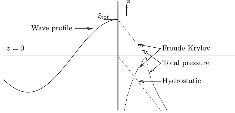
Figure 4.8: Froude-Krylov pressure.
