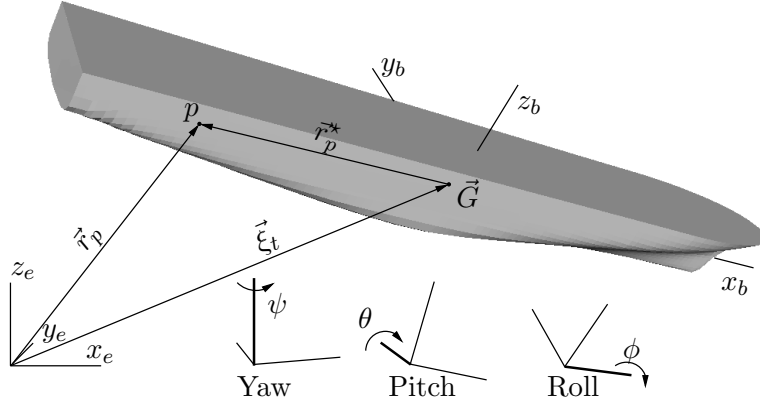
Figure 4.2: Euler transformation.
