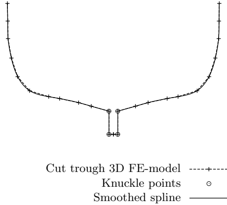
Figure 2.7: Create cross section
