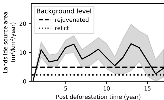
Figure 13. Deforestation-induced landslide wave. Total landslide source area ( LS_S , \text{m}^2 \text{ km}^{-2} \text{ yr}^{-1} ) as a function of time elapsed since deforestation, based on the analysis of 374 post-deforestation landslides in rocks of category III (Sect. 4.1). The grey area is the 90 % confidence interval, derived from 100 iterations of LS_S calculations (Sect. 3.2.4). The dashed and dotted line represent the overall erosion rates in rejuvenated and relict landscapes, respectively. There are not enough observations to make two separate consistent plots for rejuvenated and relict landscapes (Fig. S1 in the Supplement)
