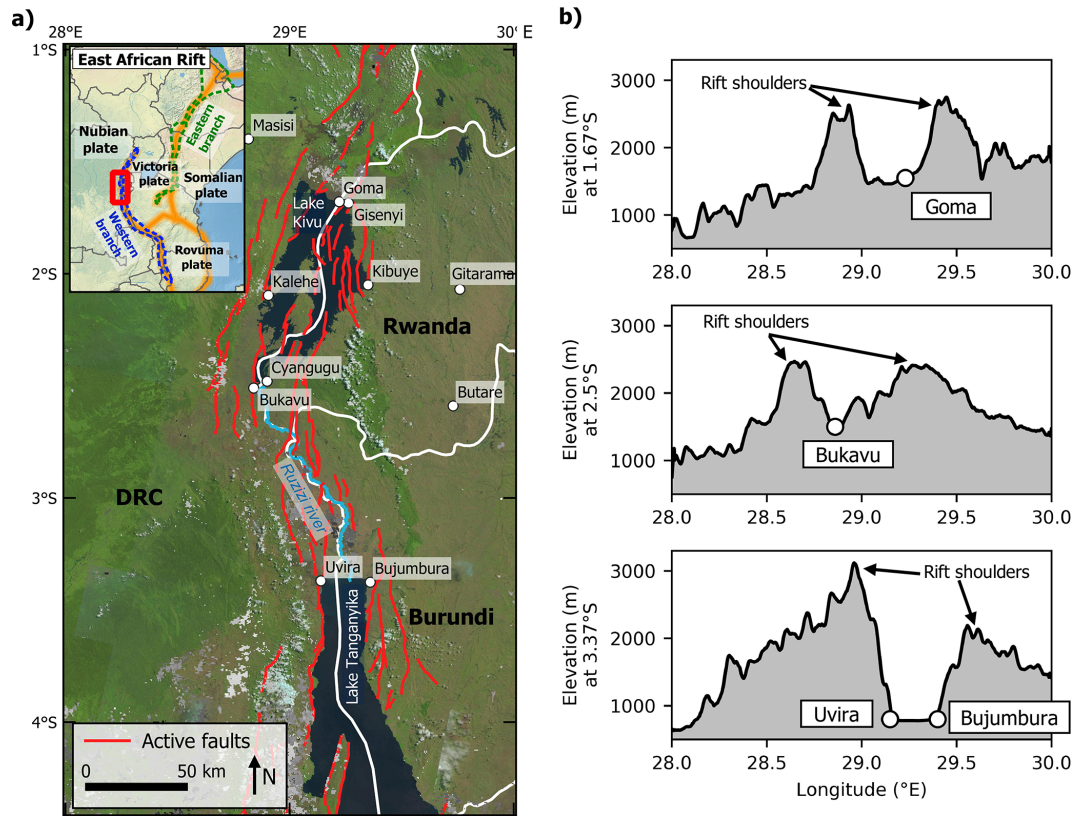
Figure 1. Overview of the North Tanganyika–Kivu (NTK) rift. (a) Extent of the studied area and active faults (Delvaux and Barth, 2010). LANDSAT-8 imagery is used as background (USGS, 2018). (b) The transects of the elevation at different latitudes illustrate the elevated rift shoulders, being the result of tectonic uplift. The four most populous cities in the area of the NTK rift (Goma, Bukavu, Uvira, Bujumbura) are located in between the rift shoulders. The transect was derived from the 30 m resolution digital elevation model (DEM) provided by the Shuttle Radar Topography Mission (SRTM) (USGS, 2006).
