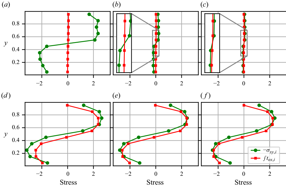
Figure 10. Shear stress \sigma_{xy,i} and integrated ocean drag \int t_{ox,i} := \Delta y \sum_{j=1}^i t_{ox,j} extracted from the DEM for (a,b,c) A_0 = 0.7 and (d,e,f) A_0 = 0.9 , and u_{o,max} values (a,d) 0.1 \text{ m s}^{-1} , (b,e) 0.5 \text{ m s}^{-1} and (c,f) 1 \text{ m s}^{-1} .
