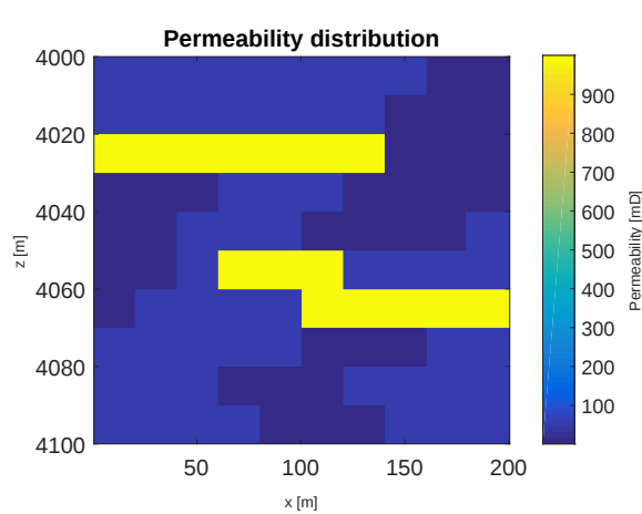
Figure 15 Permeability K_x .
