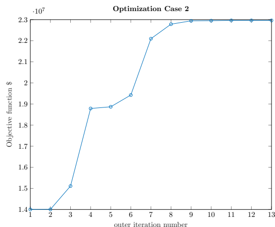
Figure 21 IDD optimization with P = 100 $/m³. Objective function is undiscounted NPV in $.
