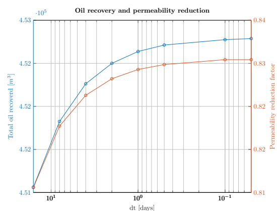
Figure 8 Cumulative oil recovery and permeability reduction as a function of time resolution for \Delta x = 1 m.
