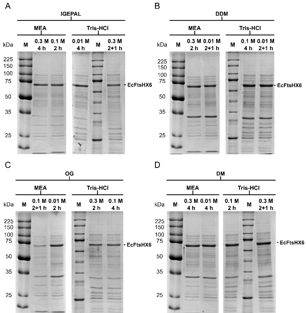
Figure 2.6 – SDS Page gels resulting from the incomplete factorial approach. They show the influence of different detergents (A – IGEPAL; B – DDM; C – OG and D – DM), buffers (MEA and Tris-HCl), salt concentrations (0.01, 0.1 and 0.3 M) and time incubation (2, 4 and 2+1 hours), during membrane solubilisation of EcFtsHX6. All the conditions are indicated on top of the gels.
