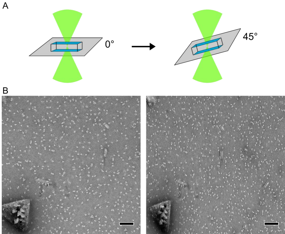
Figure 5.1 – Tilting pairs acquisition of negatively stained sample. Schematic representation of the tilt pairs acquisition inside the electron microscope at 0^\circ and 45^\circ (A). The tilt pairs were acquired using as guide the dust present on the grid by the uranyl acetate stain (left corner of both figures in B). Scale bar represents 100 nm.
