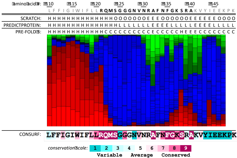
Supplementary Figure 4.6 - Structure of the ~20 aa region (amino acids in black) between the TM2 and the AAA-domain of Aquifex aeolicus FtsH, as predicted by the structure predictors SCRATCH, PREDICTPROTEIN and PRE-FOLD 3 (H: helical; E: extended; L: loop; C: coil; O: other). Residue conservation scores are obtained from the ConSurf server (scale at the bottom).
