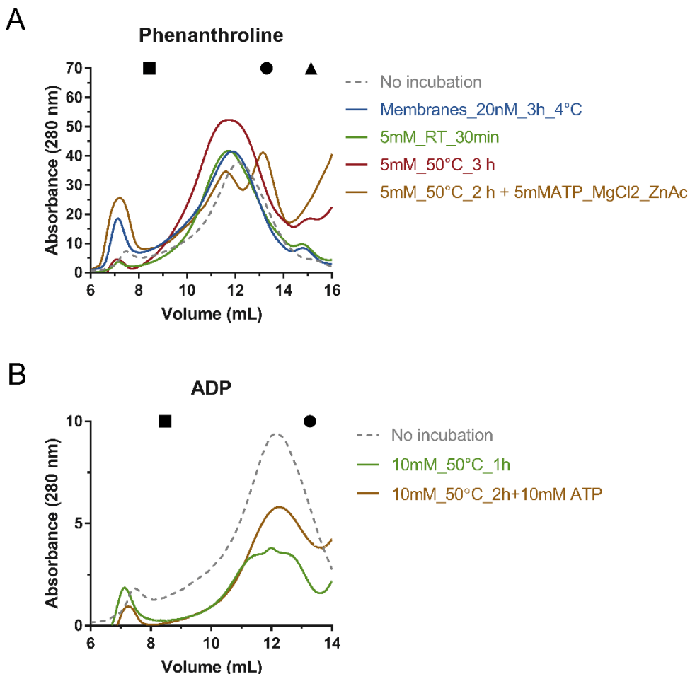
Figure 3.2 – AaFtsH size exclusion profiles after incubation with 1, 10 – phenanthroline and ADP (A and B). Only the elution profile that resulted from the HisTrap fractions incubation at 50 °C with 1, 10 – phenanthroline and ATP shows a profile different from the elution profile with no incubation (grey trace) (A). B shows the SEC elution profiles after incubating the HisTrap fractions with ADP. No significant difference is detected between conditions. The grey traces on the graphs indicate the SEC elution profile of the HisTrap fractions which were directly loaded into the Superose 6 10/300 GL column. Blue Dextran (■) is used to calculate the void volume of the column (8.47mL). The elution volumes of standard proteins used to estimate the molecular weight of the eluted fractions are shown on the top of the graph: (●) Tyroglobulin (MW: 669 kDa; V_e : 13.27 ml), (▲) Ferritin (MW: 440 kDa; V_e : 15.13 ml), (◆) Aldolase (MW: 158 kDa; V_e : 16.62 ml) and (★) Ovalbumin (MW: 44kDa; V_e : 17.76 ml).
