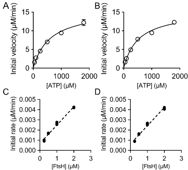
Figure 4.6 - ATPase and protease activity assays. A, B – Steady-state velocities for the ATP hydrolysis by 0.25 \mu\text{M} AaFtsH dodecamers (A) and hexamers (B). The average and SD of three replicas for each reaction are plotted (SD bars are not visible for some points due to their small sizes). C, D – Initial velocities of proteolysis of 50 \mu\text{M} resorufin-labelled casein by AaFtsH dodecamers (C) and hexamers (D) as a function of AaFtsH concentration. All the reactions were measured three times and all points are plotted.
