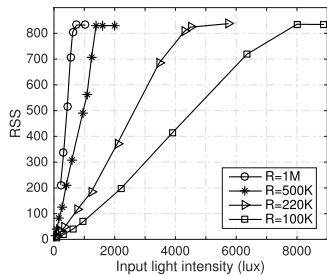
Fig. 9. Measured RSS using a PD and different feedback resistors R .
