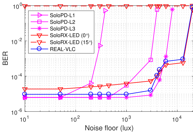
Fig. 16. The BER performance under different light conditions. In this figure, ‘SoloRX-LED (0°)’ denotes the scenario where the RX-LED and the transmitter are well aligned. Similarly, ‘SoloRX-LED (15°)’ denotes the scenario that the RX-LED and the transmitter are misaligned by an angle of 15° (the FOV of the RX-LED is 8°). The BER under REAL-VLC increases significantly to nearly 100% when the noise floor reaches 2 \times 10^4 because the RX-LED has been saturated.
