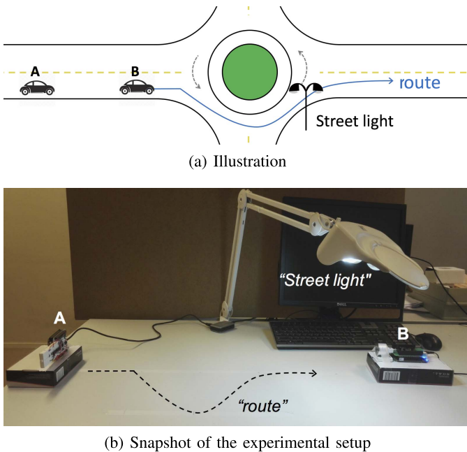
Fig. 18. Application test: route of the mobile nodes and environment setup. Two different types of LEDs are used in the experiments to support different communication distance: (i) the White LED with a FOV of 160^\circ (cf. Fig. 13), and (ii) a 3W PinYuanLighting LED with a FOV of 60^\circ .
