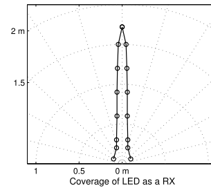
Fig. 8. Coverage of a RX-LED.
