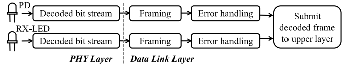
(b) Process the PD and RX-LED in parallel
