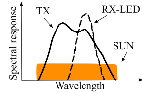
Fig. 4. RX-LED used as photodetector. Its narrow spectral response filters a large component of the noise from the sun and reduces the risk of saturation.
