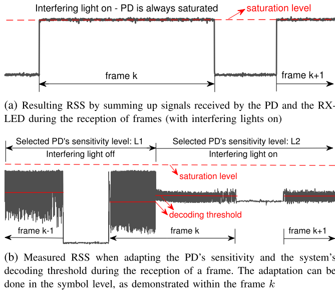
Fig. 15. Change on-the-fly re-configurations of the receiver.
