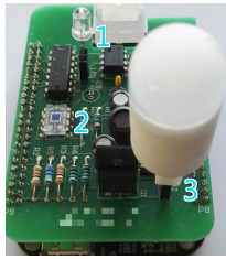
Fig. 13. The prototype of our system. ( Left ) the front-end transceiver where the three optical elements are: 1) RX-LED; 2) PD; 3) White LED. ( Right ) the key electronic components used in our system.
