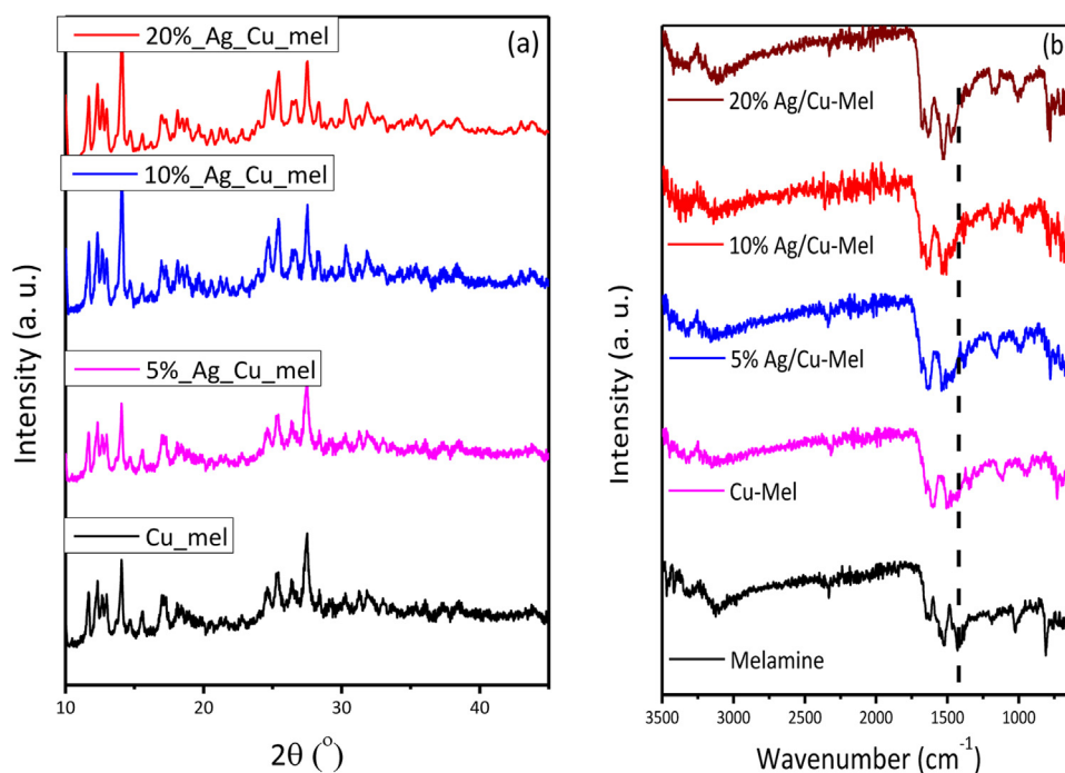
Fig. 2. (a) XRD and (b) The FT-IR of Cu-Mel, 5-Ag-Cu-Mel, 10 % Ag-Cu-Mel and 20 % Ag-Cu-Mel.
