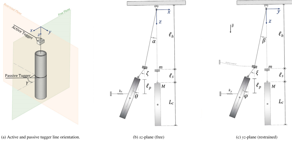
Fig. 6. Schematics of the numerically simulated triple spherical pendulum system analogue.
