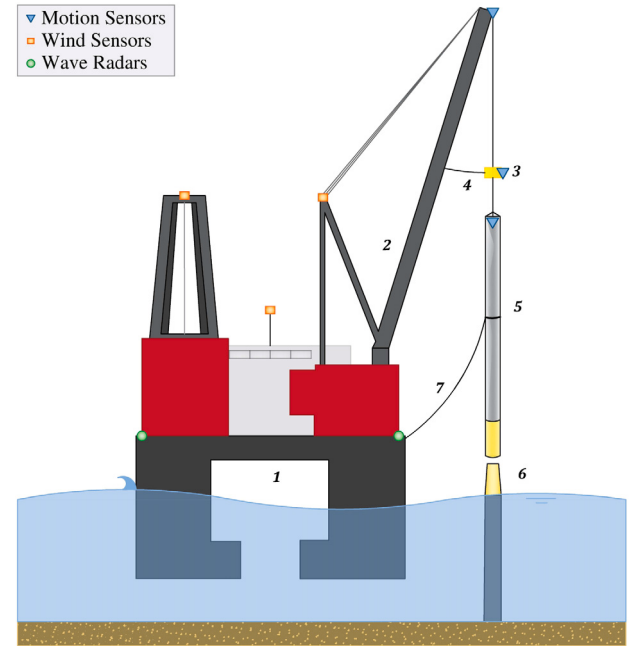
Fig. 2. Schematic diagram of the tower installation: 1. Floating vessel, 2. Heavy lift crane, 3. Lifting block/hook, 4. Active (damping) tugger line, 5. Wind turbine tower, 6. Monopile head and 7. Passive (manual) tugger line. Symbols indicate motion sensors, wind sensors, and wave radars.
