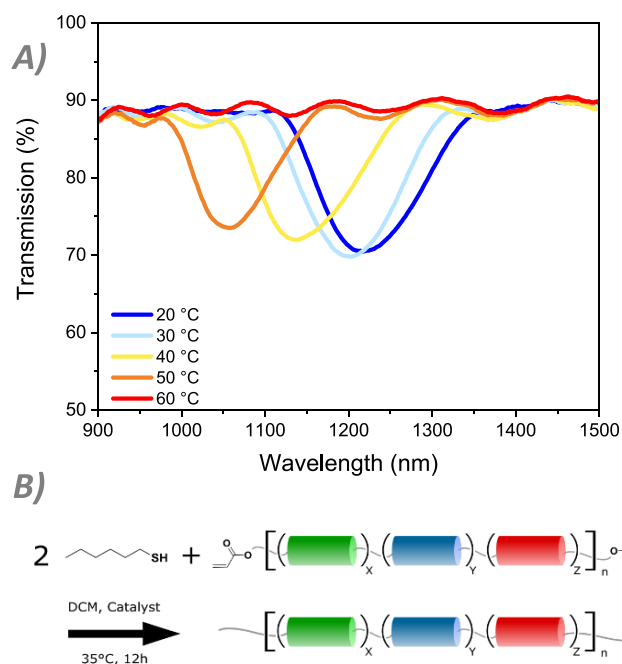
Figure 7. (A) Temperature response of the reflection band of the thiol-modified oligomer 2 . (B) Modified reaction scheme following the same procedure as the original synthesis.
