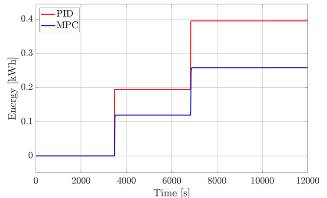
Fig. 15. PID and MPC TT energy consumption comparison.
