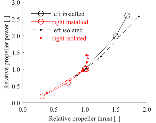
Fig. 15: The propeller performance of the left and right propeller in installed and isolated condition, relative to the installed performance of the nominal hover case.
