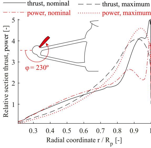
Fig. 16: Radial thrust and power distribution comparison for the nominal and maximum thrust hover cases, plotted w.r.t. the time-averaged blade performance, at \phi = 230^\circ as defined in Figure 5.
