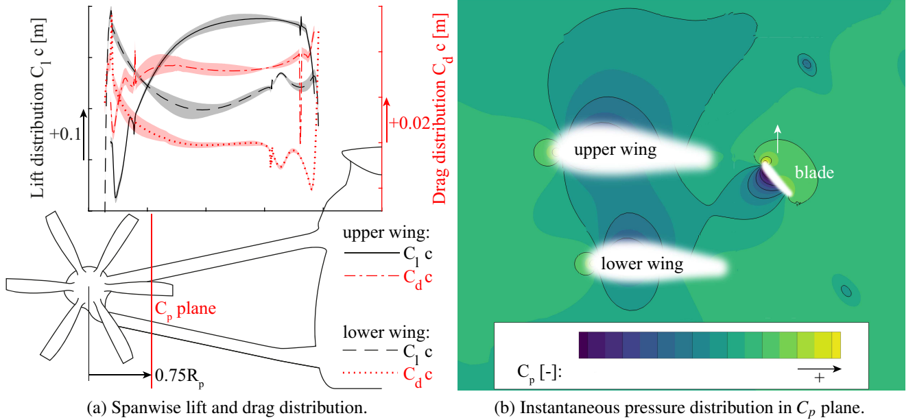
Fig. 11: The upstream effect of the left propeller on the box-wing is highlighted in the cruise condition for \delta_f = 0^\circ . The time-averaged lift and drag distribution are shown in (a) with the variation in time indicated by the shaded areas. The distribution of static pressure in a plane cutting the wings and a propeller blade is shown in (b).
