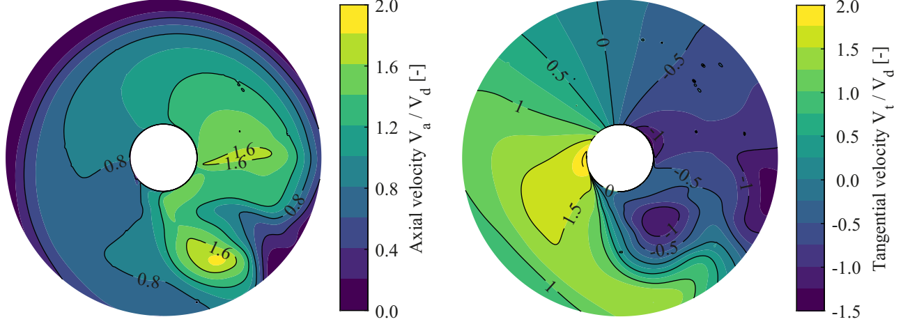
Fig. 13: Contours of time-averaged velocity components at a plane 0.18R_p upstream of the left propeller in hover.
