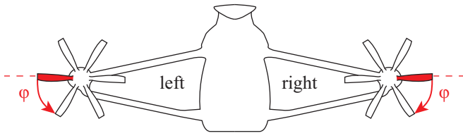
Fig. 5: Rear view of helicopter with blade phase angle definition for the left and right propeller.
