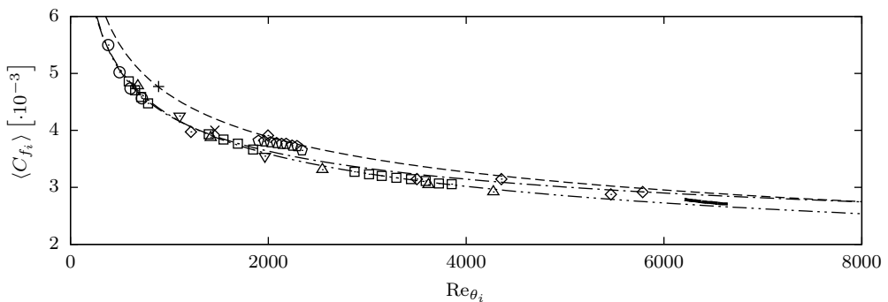
Figure 5: Incompressible skin-friction distribution. (—) Present LES ( \mathcal{G}^2 ), (----) Blasius, (-·-·-) Kármán-Schoenherr (both adopted from Hopkins & Inouye (1971)), (-·-·-) Smits et al. (1983), ( \square ) Pirozzoli & Bernardini (2011), ( \odot ) Komminaho & Skote (2002), ( \triangle ) Schlatter & Örlü (2010), ( \nabla ) Simens et al. (2009), ( \diamond ) Pirozzoli et al. (2004), ( \times ) Maeder et al. (2001), (+) Guarini et al. (2000), ( \diamond ) Coles (1953) (CAT5301, from Fernholz & Finley (1977))
