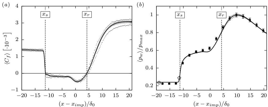
Figure 7: (a) Skin-friction and (b) wall-pressure evolution: (—) Present LES (averaged in time and spanwise direction; spanwise min and max values of the time-averaged data are indicated by the grey shaded area for the long integration time of 3805 \delta_0/U_0 and by dots for the short integration time of 446 \delta_0/U_0 ), (●) experimental static pressure measurements and (◊) mean experimental unsteady pressure measurements from Daub et al. (2015). Error-bar indications are only rough experimental estimates due to Willems (2016).
