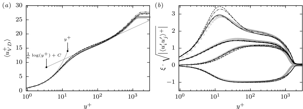
Figure 4: (a) Van Driest transformed mean velocity profile and (b) rms of Reynolds stresses with density scaling \xi = \sqrt{\langle \rho \rangle} / \langle \rho_w \rangle for all grid resolutions at Re_\tau = 1523 and (x - x_{imp}) / \delta_0 = -15.25 : (----) \mathcal{G}^1 , (-·-·-) \mathcal{G}_z^1 , (—) \mathcal{G}^2 , (-·-·-) \mathcal{G}_x^2 . See table 2 for reference. ( \odot ) Incompressible DNS data adopted from Schlatter & Örlü (2010) at Re_\tau = 1271 .
