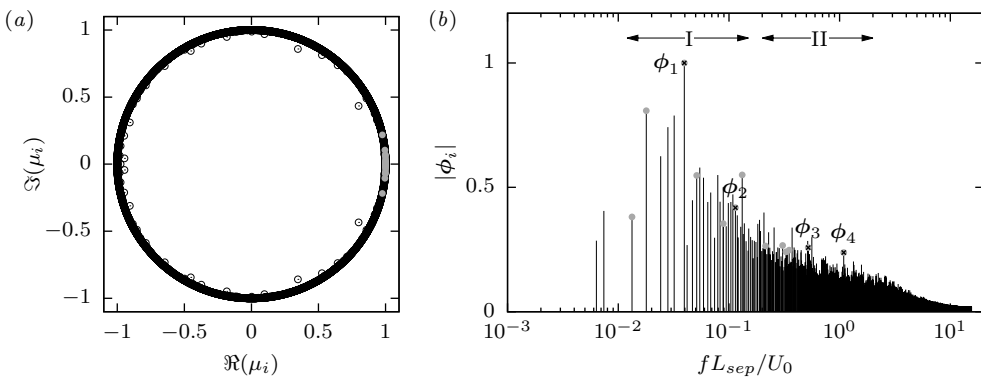
Figure 18: (a) Spectrum of eigenvalues resulting from the standard DMD algorithm. (b) Normalised magnitudes of the DMD modes. (●) indicate a SPDMD subset of N_{sub} = 13 modes.
