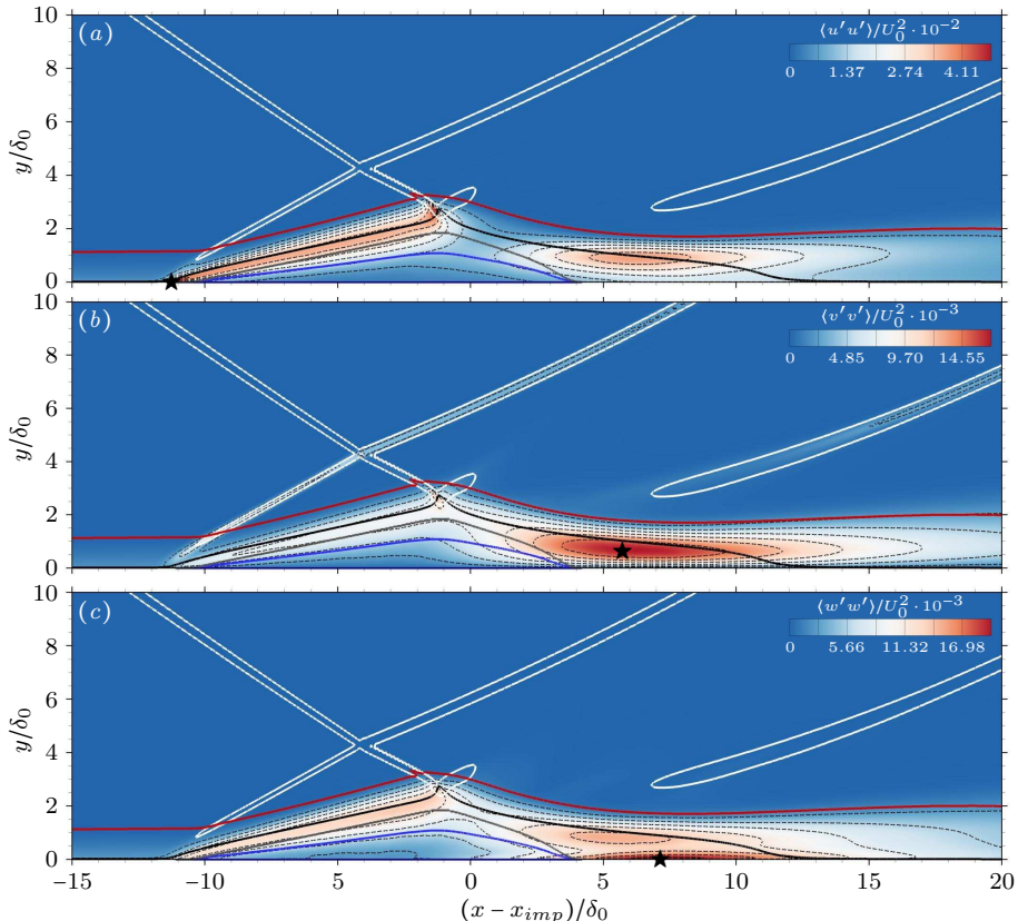
Figure 8: Time- and spanwise-averaged Reynolds normal stress components. The shock system is visualised by isolines of pressure gradient magnitude |\nabla p| \delta_0 / p_\infty = \{1.08, 3.28\} . (—) \delta , (—) \langle Ma \rangle = 1 , (—) \langle u \rangle = 0 , (—) dividing streamline y_{ds} . A star ( \star ) indicates the location of maximum contour level. Eight discrete contour levels are shown by dashed lines.
