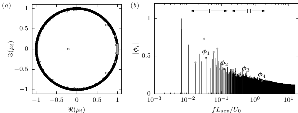
Figure 21: (a) Spectrum of eigenvalues resulting from the standard DMD algorithm. (b) Normalised magnitudes of the DMD modes. (●) indicate a SPDMD subset of N_{sub} = 17 modes.
