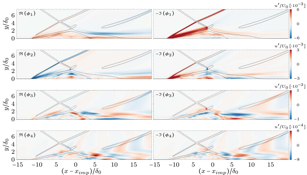
Figure 20: Real and imaginary part of DMD modes showing contours of modal velocity fluctuations u'/U_0 . Left column: \Re(\phi_i) . Right column: -\Im(\phi_i) . Refer to figure 18 for the mode selection. For clarity, the mean shock system, the mean sonic line and the mean dividing streamline are superimposed by black solid lines.
