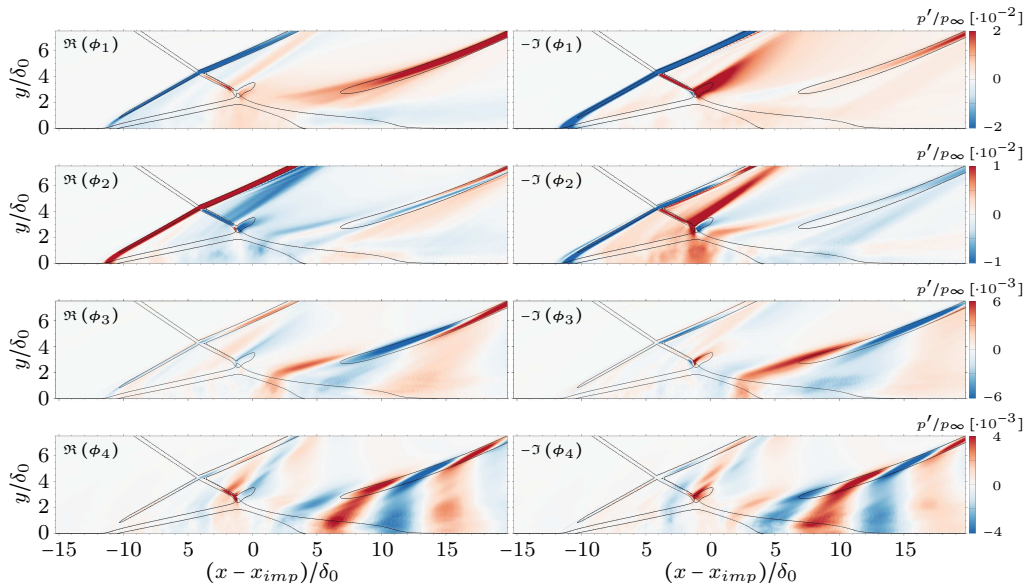
Figure 19: Real and imaginary part of DMD modes showing contours of modal pressure fluctuations p'/p_\infty . Left column: \Re(\phi_i) . Right column: -\Im(\phi_i) . Refer to figure 18 for the mode selection. For clarity, the mean shock system, the mean sonic line and the mean dividing streamline are superimposed by black solid lines.
