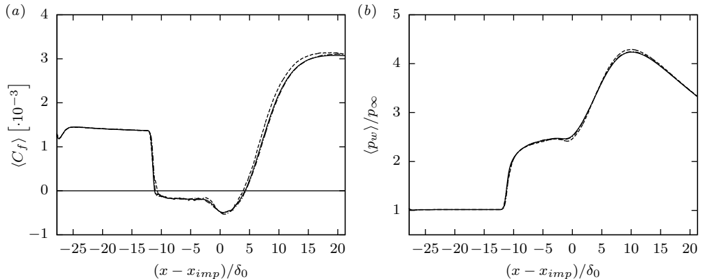
Figure 3: Domain-sensitivity study with respect to (a) skin-friction coefficient and (b) wall-pressure evolution. Reported quantities are time- and spanwise-averaged. ( - - - - ) \mathcal{D}^1 , ( — ) \mathcal{D}^2 , ( - · - · - ) \mathcal{D}^3 . See table 3 for reference.
