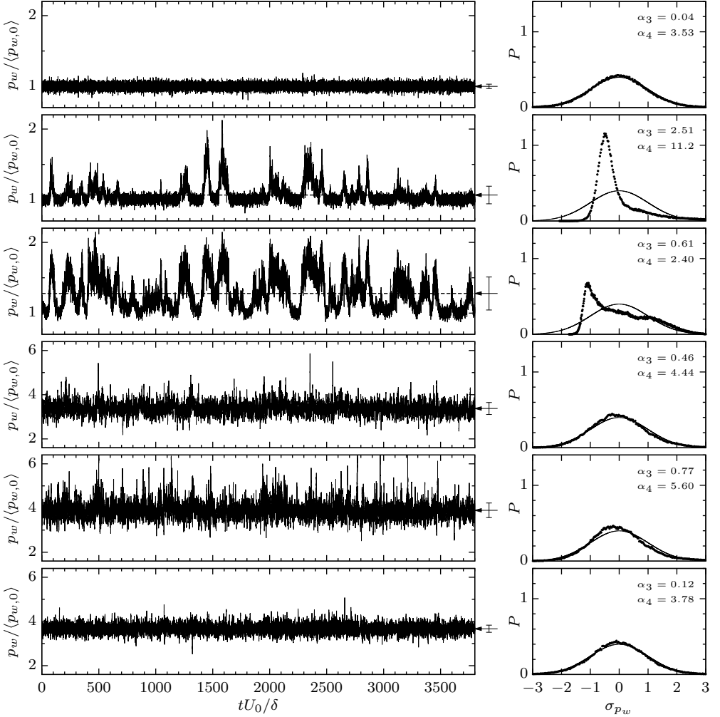
Figure 15: Wall-pressure signals (left) and corresponding normalised probability density distributions (right) evaluated at (x - x_{imp})/\delta = \{-17.74, -11.66, -11.34, 4.25, 6.61, 17.18\} . Refer to the text and figure 14 for a physical interpretation of the wall-pressure positions. The mean wall-pressure is indicated by a horizontal dashed line. Arrows together with vertical bars indicate the mean wall-pressure and its standard deviation. Values of skewness \alpha_3 and flatness \alpha_4 coefficients and a Gaussian distribution are included for reference.
