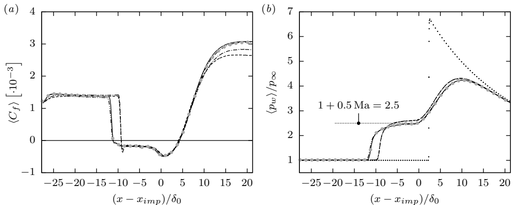
Figure 2: Grid-sensitivity study with respect to (a) skin-friction coefficient and (b) wall-pressure evolution. Reported quantities are time- and spanwise-averaged. (----) \mathcal{G}^1 , (-·-·-) \mathcal{G}_z^1 , (—) \mathcal{G}^2 , (-·-·-·) \mathcal{G}_x^2 , (●) \mathcal{G}^2 averaged over 446 \delta_0/U_0 , (·····) inviscid interaction. The plateau pressure prediction according to Zukoski (1967) is also shown. See table 2 for reference.
