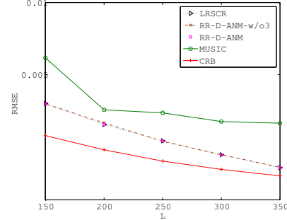
(b) RMSE vs. L with \text{SNR}=5\text{dB}
