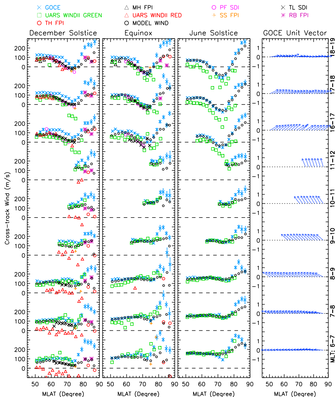
Figure 7. Average quiet time cross-track wind observed by GOCE and computed from FPIs, SDIs, and WINDII data as a function of season and magnetic latitude (MLAT, 2^\circ bin), for successive 1 h magnetic local time (MLT) bins around the dusk and dawn time sectors. Black circular symbols show modeled average cross-track wind along the GOCE orbit. The rightmost column shows the direction of the average GOCE cross-track unit vector as function of magnetic latitude. Magnetic north (east) is at the top (right) of the page.
