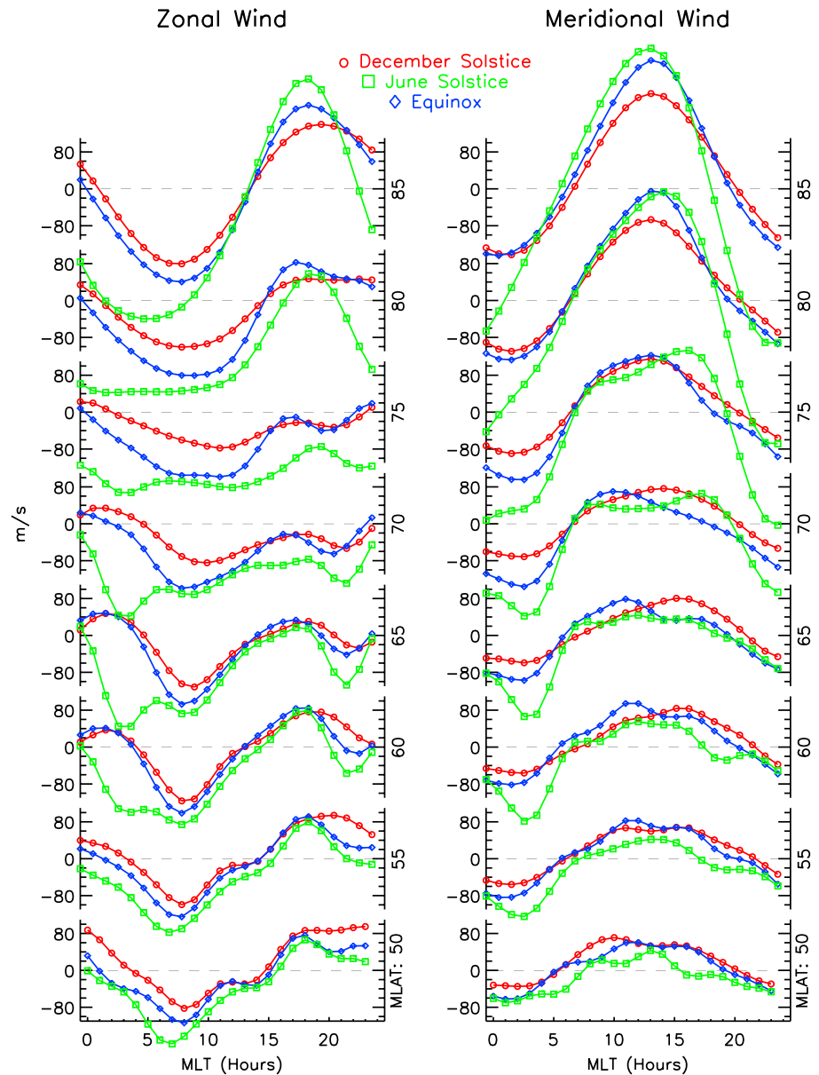
Figure 10. Interseasonal comparison of quiet time modeled average neutral (left) zonal and (right) meridional winds as a function of magnetic local solar time at various northern high latitudes (annotated on the right).
