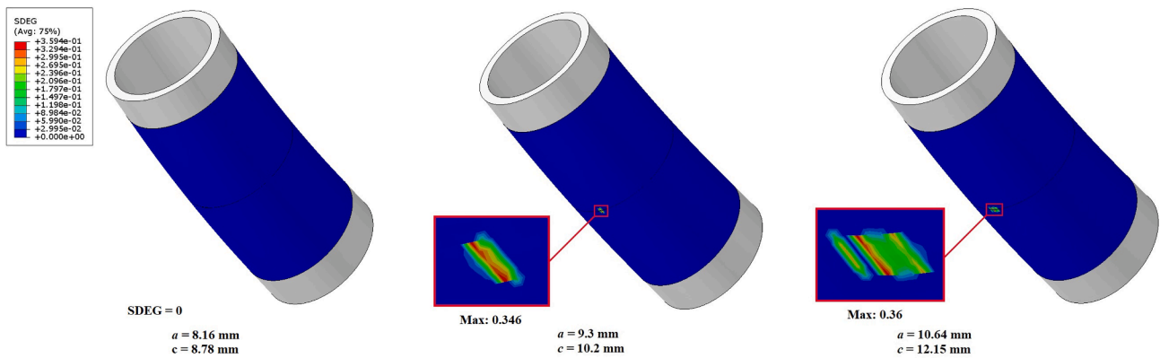
Fig. 10. Interfacial stiffness degradation with different crack sizes along with the crack growth process under the bending moment of 6.0385 \times 10^7 kN·m
