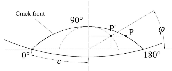
External surface crack
