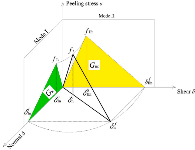
Fig. 2. The mixed-mode traction-separation law.
