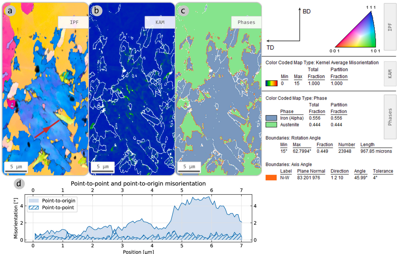
Fig. 3–8. (a) Inverse Pole Figure (IPF) of bainitic island within interface layer obtained with a step size of 70 nm. (b) Kernel Average Misorientation (KAM) showing grain boundaries larger than 15^\circ in white. (c) Phase map highlighting boundaries that match with N-W orientation relationship. (d) Point-to-point and point-to-origin misorientation profile at location marked in (a). The legend includes reference axis to maps, IPF, KAM and Phase map color legends, as well as total grain length density of boundaries matching the orientations of interest.
