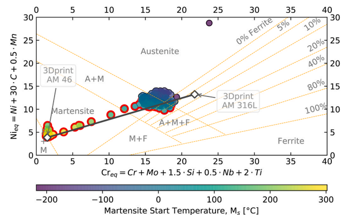
Fig. 3–3. Schaeffler diagram including Cr_{eq} and Ni_{eq} of values obtained from a line scan as measured by EPMA, see Fig. 3b. Color indicates M_s temperature. Red outlining indicates M_s temperature above 0 °C.
