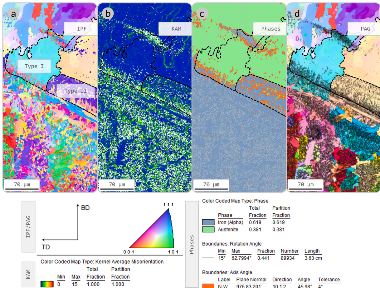
Fig. 3–7. (a) Inverse Pole Figure (IPF) of boundary region between last layer of HSLA steel and the interface layer, obtained with a step size of 700 \text{ nm} . (b) Kernel Average Misorientation (KAM). (c) Phase map showing grain boundaries larger than 15^\circ in white and boundaries that match the N-W orientation relationship. (d) Parent austenite grain reconstruction overlaid on the Image Quality map. Legend includes reference axis to maps, IPF, KAM, Phase map color legends and large angle grain boundary length.
