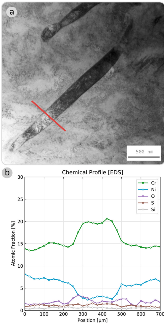
Fig. 3-10. (a) TEM-BF image showing interdentritic bcc phase entirely contained within an fcc matrix indicating the location of the EDS chemical profile shown in (b).
