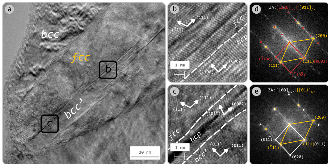
Fig. 3-13. (a) HREM of bcc phases surrounding the austenite phase with a martensite plate originating from its grain boundary, Zone Axis [001] bcc || [011] fcc. (b) Higher magnification region including HCP martensite (c) Higher magnification region including bcc martensite, hcp transition region and fcc matrix (d) FFT of region b (e) FFT of region c.
