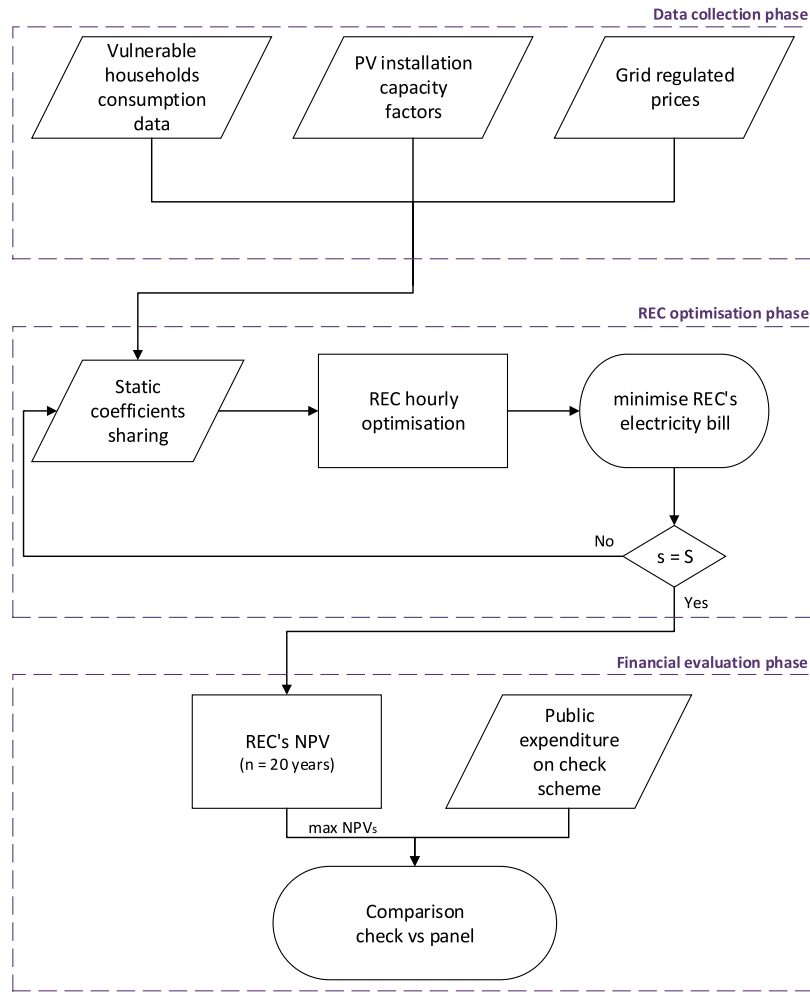
Fig. 1. Methodology workflow.
